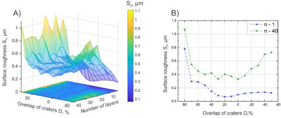
Fig. 4.6 (A) Surface roughness evolution when different overlaps of the craters are used. (B) Surface roughness dependence on the overlap value in single and multi-scan (40) cases. Processing parameters: Fluence F = 26.1 \text{ J/cm}^2 , angle of rotation \alpha = 73^\circ , wavelength \lambda = 1030 \text{ nm} . The uncertainty of layer positioning of a maximum magnitude \Delta \geq dx was maintained.
