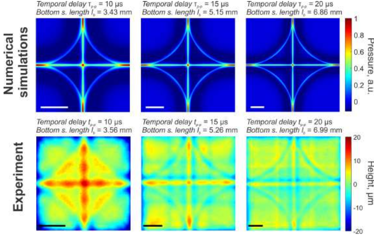
Fig. 6.8 Pressure maps of surfaces with different bottom side lengths l_b and pulse repetition periods \tau_{p-p} generated using the numerical model presented in the study (top row). The amplitudes in each pressure map are normalized. Height maps of the bottom surfaces of deep ablated rectangular cavities with bottom side lengths l_b and pulse repetition periods \tau_{p-p} (bottom row). Laser processing parameters used: fluence F = 18.2 \text{ J/cm}^2 , overlap of the craters \Omega = 20 \% , number of scans N = 775 , engraved depth h = 820 \text{ μm} .
