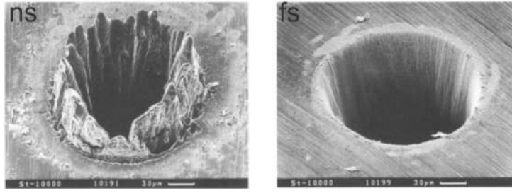
Fig. 1.15 A comparison of holes drilled using ns pulses (on the left) and fs pulses (on the right) [145].
