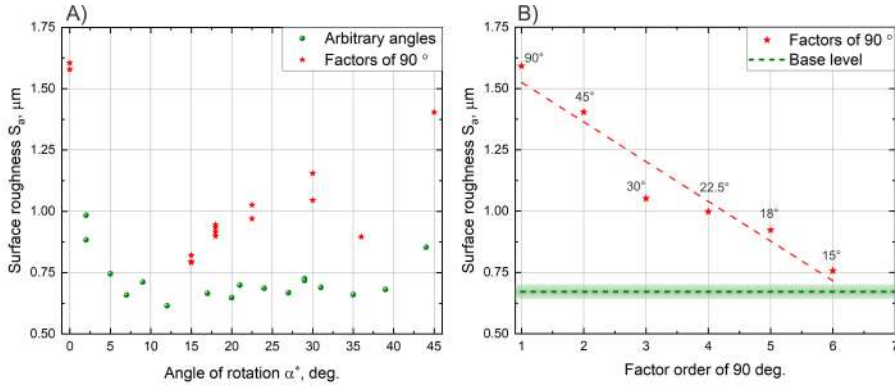
Fig. 4.2 (A) The surface roughness dependence on the angle ( \alpha ) of layer rotation, when surface is scanned 30 times. Two distinctive angle categories are depicted: arbitrary angles and factors of 90^\circ . (B) The dependence of the surface roughness on the angles of rotation that are factors of 90^\circ . The fit is presented as a red dashed line, whereas the base level formed of arbitrary angles is presented as a green dashed line with a standard deviation ( 1\sigma ) shown as a green area. Processing parameters: Fluence F = 52 \text{ J/cm}^2 , overlap of the craters \Omega = 20 \% , wavelength \lambda = 1030 \text{ nm} .
