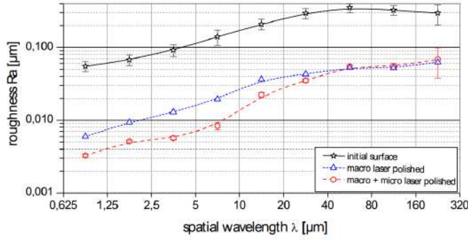
Fig. 7.2 Roughness dependence on spatial wavelength. Black curve represents initial surface roughness, blue curve - after macro laser polishing, while red - after combined macro and micro laser polishing procedures [26].
