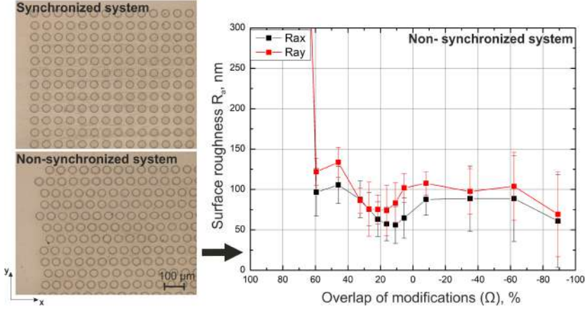
Fig. 3.8 Surface morphology after single-pass ablation with synchronized system (top left) and with non-synchronized (bottom left). Surface roughness as a function of modification overlap in the non-synchronized system (right). Results achieved with 1 st experimental system configuration (see section 2.1), E_p = 173 \mu\text{J} , \lambda = 1030 \text{ nm} .
