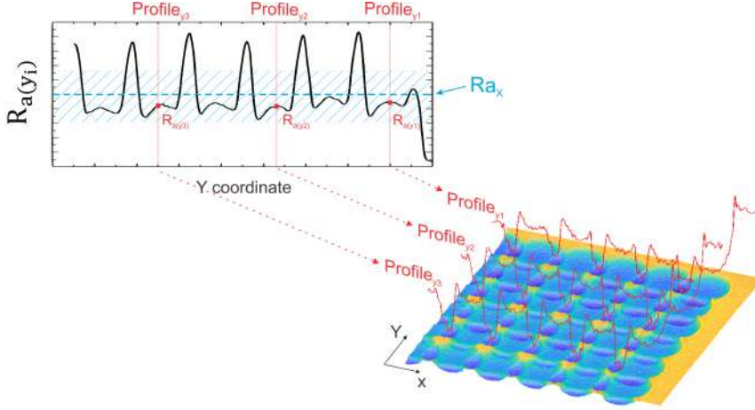
Fig. 3.2 Scheme explaining how areal roughness parameter is derived. The topography of a sample after single scan machining is examined. Red curves represent profiles at discrete locations. R_a parameter dependence on Y coordinate is calculated in preferred direction. The average of all R_a values is then an areal roughness parameter in a perpendicular direction Ra_x . Tilted blue lines represent the range of one standard deviation.
