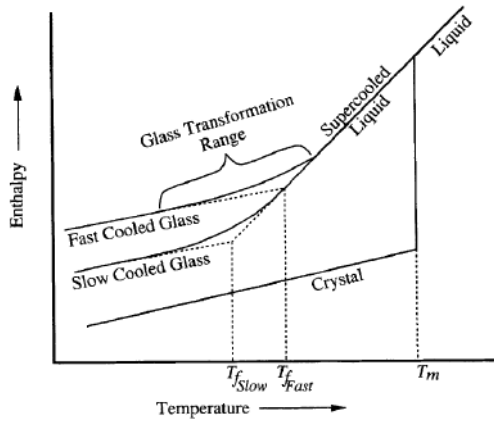
Fig. 1.13 Effect of temperature on the enthalpy of a glass forming melt. T_{f,slow} here is fictive temperature for slow cooled melt, whereas T_{f,fast} is a fictive temperature for fast cooled melt. T_m denotes melting temperature [139].
