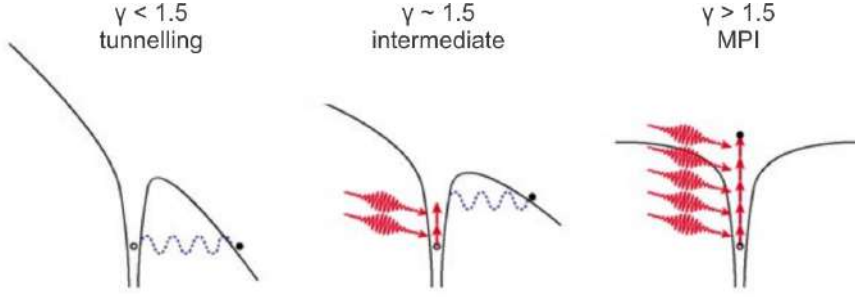
Fig. 1.8 Schematic diagram of the photoionization of an electron in an atomic potential for different values of the Keldysh parameter. In a solid, the electron is promoted from the valence to the conduction band, rather than ionized [108].
