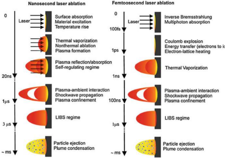
Fig. 1.14 Approximate time scales of nanosecond and femtosecond energy absorption and laser ablation along with various processes happening during and after the laser pulse [126].
