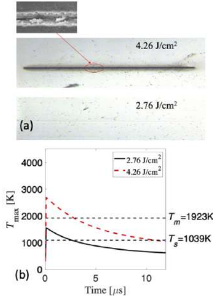
Fig. 7.7 (a) Microscopy images of line-scan-based processing, and (b) predicted surface temperature evolution for two laser fluences [231].
