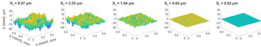
Fig. 5.1 Topographies of initial surfaces with varying surface roughness (see roughness values S_q at the top left corner above each topography). The surfaces were prepared using conventional mechanical grinding means.
