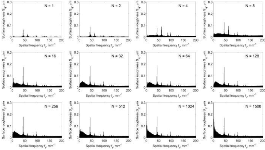
Fig. 5.5 Spatial spectra of processed surfaces after different numbers of scans ( N ). Processing was performed on a surface of an optical quality roughness level. Laser processing parameters: fluence F = 12.2 \text{ J/cm}^2 , scanning speed v = 2324.8 \text{ mm/s} , scanning pitch dx = 23.24 \text{ } \mu\text{m} , overlap of the craters \Omega_{x,y} = 20 \text{ } \% .
