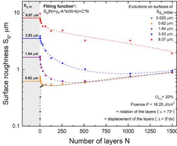
Fig. 5.8 Surface roughness S_q dependence on the number of scans N , when laser processing is performed on surfaces with varying initial roughness ( S_{q\_int} values given in the legend). Dots represent raw data, while the dashed lines represent the fit. The fitting function is outlined in the upper-left corner of the figure (except for the case S_{q\_int} = 0.02 \mu\text{m} ; see the text for details). Laser processing parameters: fluence F = 16.25 \text{ J/cm}^2 , scanning speed v = 2324.8 \text{ mm/s} , scanning pitch dx = 23.24 \mu\text{m} , overlap of the craters \Omega_{x,y} = 20 \% .
