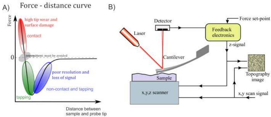
Fig. 1.7 Force - distance curve (A). The curve shows the force between the surface and the probe tip dependence on the distance between the two. Different color areas denote different modes AFM can be operated in. Schematic diagram of an atomic force microscope operating in contact mode (B) [94].
