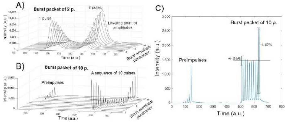
Fig. 7.3 The dependence of the intensity of the sub-pulses in the burst versus the envelope parameter when a single pulse is divided into 2 sub-pulses (A) and into 10 sub-pulses (B). Amplitudes of a leveled burst packet of 10 sub-pulses are displayed in (C).
