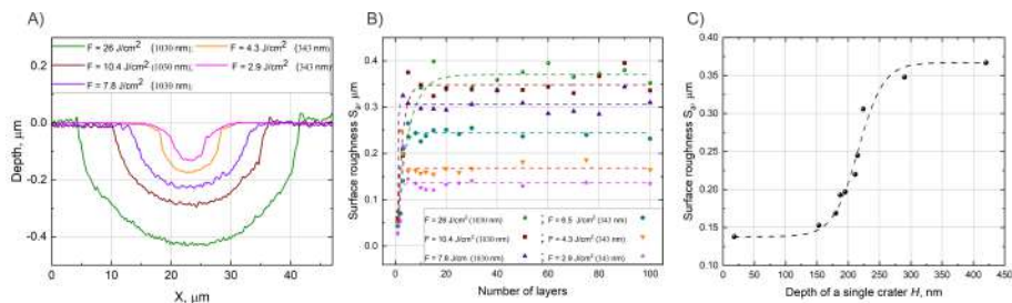
Fig. 4.7 (A) Cross sections of the craters produced using different pulse energies and wavelengths. (B) Surface roughness evolutions when utilizing craters of different dimensions. (C) Surface roughness dependence on the depth of a single crater after 100 scans when the stabilization of surface roughness is reached. Dots represent experiment data, dashed line - fit of the data. The scanning speed was adjusted to maintain the optimal overlap ( \Omega = 20\% ) in all the cases. In addition, each layer was rotated by 73^\circ . The uncertainty of layer positioning of a maximum magnitude \Delta \geq dx was maintained.
