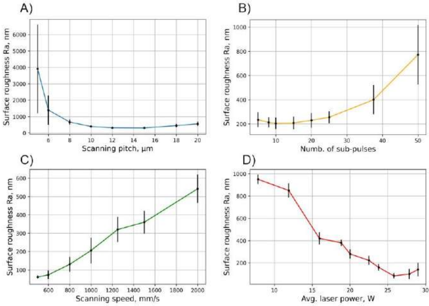
Fig. 7.4 Surface roughness after polishing ablated samples dependencies on different polishing parameters. Other fixed parameters in case of (A): P = 29 W, N_p = 10 and v = 1000 mm/s; in case of (B): P = 19 W, dy = 10 μm and v = 1000 mm/s; in case of (C): P = 25.8 W, dy = 10 μm and N_p = 10 ; and in case of (D): v = 1000 mm/s, dy = 10 μm and N_p = 5 .
