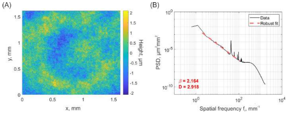
Fig. 2.4 A typical laser-processed surface topography (A). Averaged PSD versus spatial frequency f_r representation in a log-log format (B). The black curve is the raw data, while the red line represents the fit. \beta , H , and D are the parameters used in the fractal dimension calculation.
