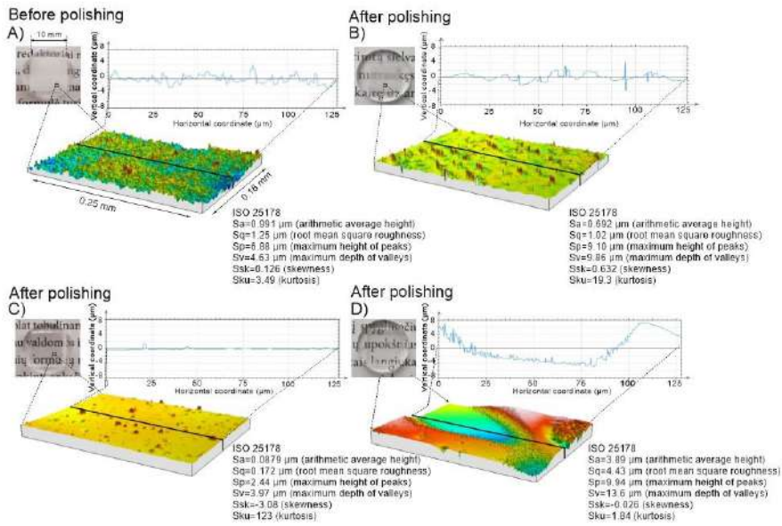
Fig. 7.5 Surface before laser polishing (A). Surface after single scan laser polishing with bursts of femtosecond pulses, with P = 12 \text{ W} , v = 1000 \text{ mm/s} , dy = 5 \mu\text{m} and N_p = 10 (B); P = 29 \text{ W} , v = 1000 \text{ mm/s} , dy = 10 \mu\text{m} and N_p = 10 (C); and P = 29 \text{ W} , v = 1000 \text{ mm/s} , dy = 5 \mu\text{m} , N_p = 10 (D).
