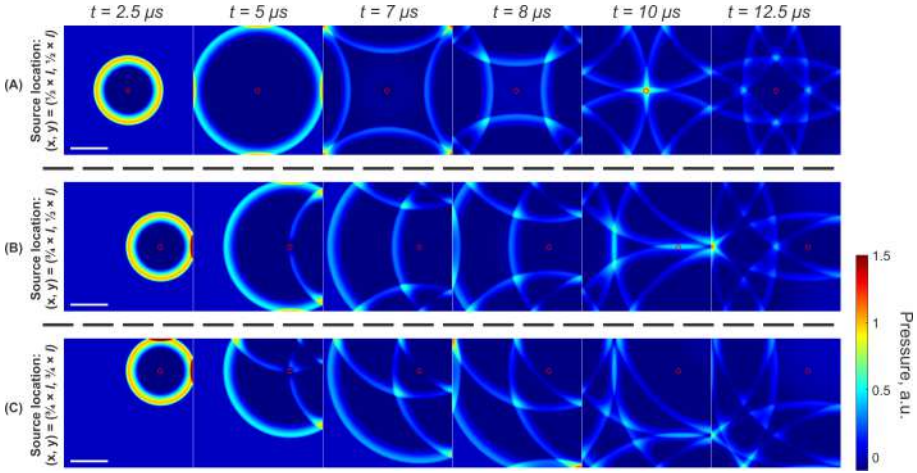
Fig. 6.6 Pressure distributions of a propagating acoustic wave at different time delays (2.5 ; 5 ; 7 ; 8 ; 10 ; 12.5 \mu\text{s} ) after initiation. Parts A, B, and C illustrate scenarios with a single source located at different positions (indicated by a red circle). Initial peak amplitude equals 1. The scale bar represents 1 mm in length and variable l stands for a side length of a rectangular cavity.
