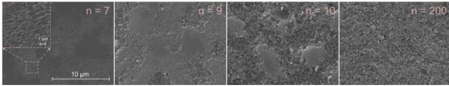
Fig. 4.8 SEM images of the ablated regions produced after different numbers of scans. Processing parameters: fluence F = 2 J/cm 2 , overlap of the craters \Omega = 20\% , angle of rotation \alpha = 73^\circ , wavelength \lambda = 343 nm. The uncertainty of layer positioning of a maximum magnitude \Delta \geq dx was maintained.
