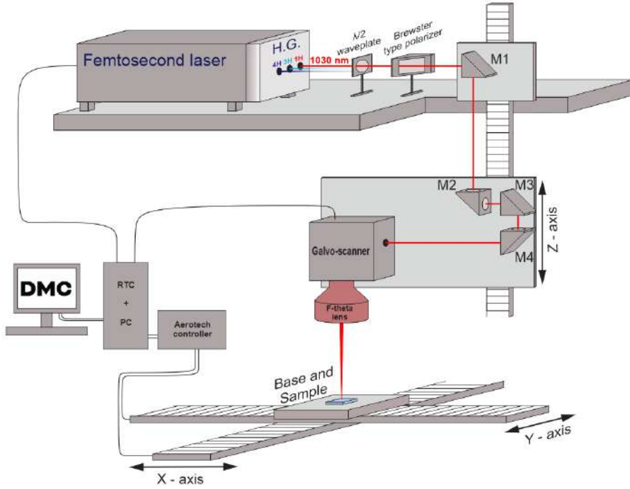
Fig. 2.1 Conceptual layout of the generalized experimental setup. H.G. stands for harmonic generator unit, M denotes different mirrors. RTC stands for "Real Time Controller" (Manufactured by ScanLab) and is used for the control of galvo-scanner and trigger of laser's pulse picker unit. PC here denotes personal computer, whereas DMC (Manufactured by Direct Machining Control) is a software that controls all active units within the experimental setup.
