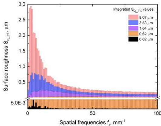
Fig. 5.2 Spatial spectra of initial surfaces with varying surface roughness levels.
