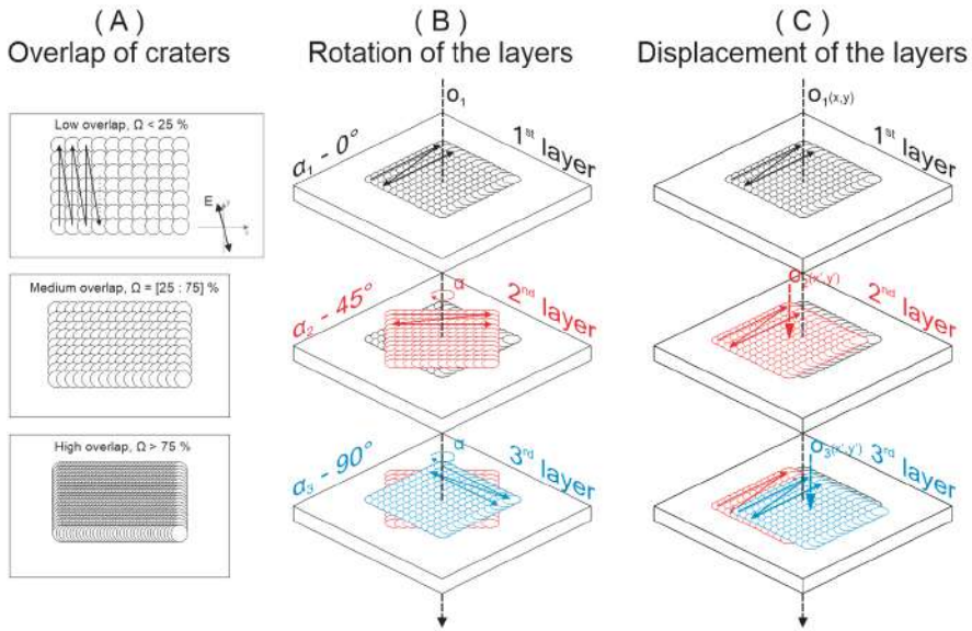
Fig. 2.2 The visual representation of different scanning algorithms used in the thesis. (A) the changing of the overlap of the craters \Omega . The E vector represents linear polarization orientation, which was maintained during all experiments. (B) the rotation of the layers, where \alpha is the angle of rotation and \alpha_n is the cumulative angle. (C) the displacement of the layers, where O_n is the central point of the scanned pattern for each layer. Different colors stand for different layers.
