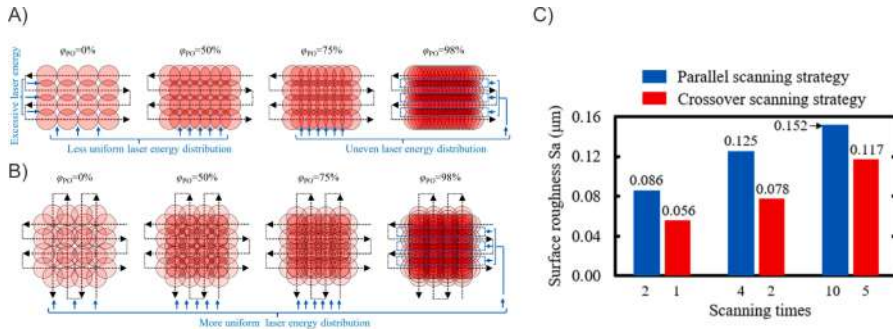
Fig. 1.20 Schematic diagram of the prototype of (A) parallel scanning strategy and (B) crossover scanning strategy with the line overlap rate of 60% and the pulse overlap rates ranging from 0 % to 98 %. Part (C) presents the statistics of the surface roughness ( S_a ) values achieved on the machined copper workpiece using the two scanning strategies [172].
