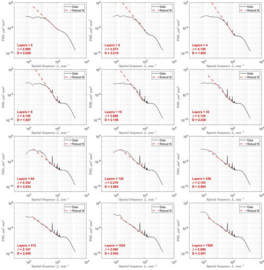
Fig. 5.10 Averaged PSD dependencies on radial spatial frequency f_r in a log-log representation of laser-processed surfaces after different numbers of scans. The initial surface roughness of the surface S_{q\_int} = 1.64 \mu\text{m} . The black curve represents raw data, while the red dashed line is a fit over a selected region of frequencies (for more detail see section 2.4). \beta here is a scaling exponent, and D is the fractal dimension.
