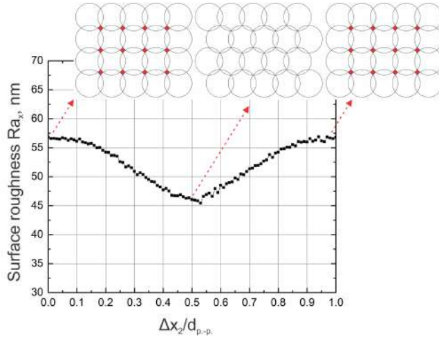
Fig. 3.9 Surface roughness dependence on the shift of every 2 nd line, when pulse distance of 32 \mu\text{m} is maintained. On x axis shift between consecutive lines \Delta x_2 divided by the pulse distance is plotted. Used system configuration – 1 (see section 2.1), E_p = 173 \mu\text{J} , \lambda = 1030 \text{ nm} . Data of numerical simulations.
