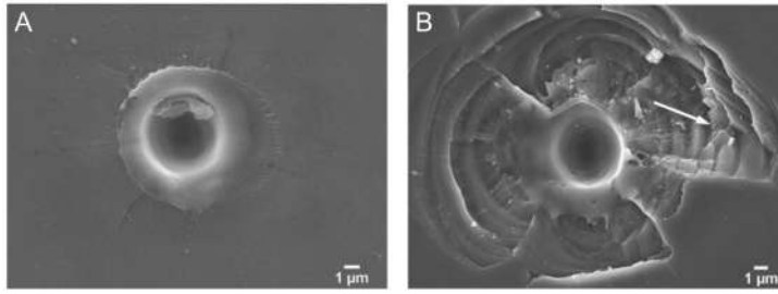
Fig. 1.16 Craters generated on sapphire with a stationary laser beam at a frequency of 1 kHz. (A) 30 \mu\text{J} and 20 pulses, (B) 50 \mu\text{J} and 40 pulses [155].
