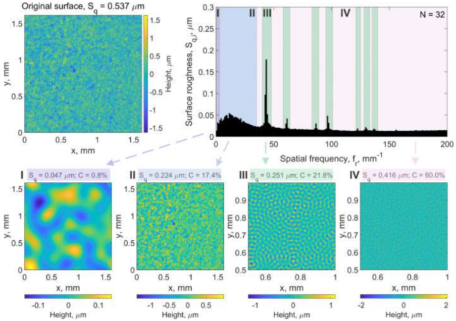
Fig. 5.7 Surface topography and its corresponding spatial spectrum after 32 laser scans applied on an initially smooth surface (top). Laser processing parameters were: fluence F = 12.2 \text{ J/cm}^2 , scanning speed v = 2324.8 \text{ mm/s} , scanning pitch dx = 23.24 \mu\text{m} , and crater overlap \Omega_{x,y} = 20 \% . The bottom part of the figure presents the surface topographies corresponding to different texture components identified in the spatial spectrum. Region I (violet) represents laser-induced waviness, region II (blue) corresponds to low-spatial-frequency components introduced by the scanning strategy, region III (green) contains the spectral peaks associated with the scanning pitch, and region IV (pink) represents the spectral background. The S_q value shown above each topography denotes the root-mean-square roughness of the corresponding texture component, while C indicates its percentage contribution to the overall surface roughness.
