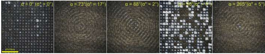
Fig. 4.3 Color images of surface structures induced by scanning the surface 30 times with different angles of rotation ( \alpha ). Fluence F = 52 \text{ J/cm}^2 , overlap of the craters \Omega = 20 \% , wavelength \lambda = 1030 \text{ nm} .
