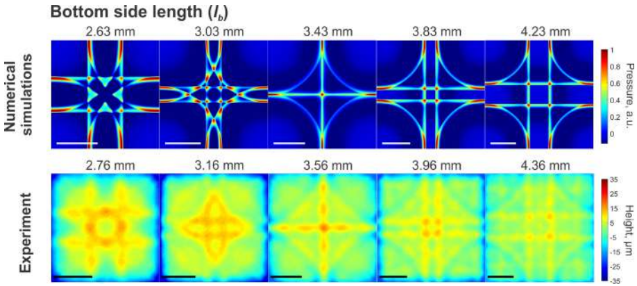
Fig. 6.7 Pressure maps of surfaces with different bottom side lengths of l_b generated using the numerical model presented in the study (top row). The amplitudes in each pressure map are normalized. Height maps of the bottom surfaces of deep ablated rectangular cavities with bottom side lengths of l_b (bottom row). Laser processing parameters used in the experiments are detailed in figure 6.3 caption.
