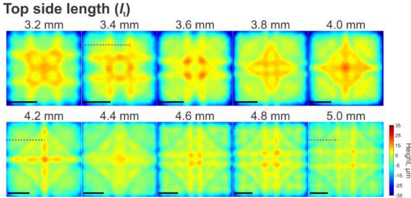
Fig. 6.3 Height maps of the bottom surfaces of deep ablated rectangular cavities with top side lengths of l_t . Laser processing parameters used: fluence F = 18.2 \text{ J/cm}^2 , scanning speed v = 2325 \text{ mm/s} , scanning pitch dy = dx = 23.3 \text{ }\mu\text{m} , number of scans N = 775 , engraved depth h = 820 \text{ }\mu\text{m} . The black bar indicates a length of 1 \text{ mm} . The dashed purple line indicates the length of 1.78 \text{ mm} .
