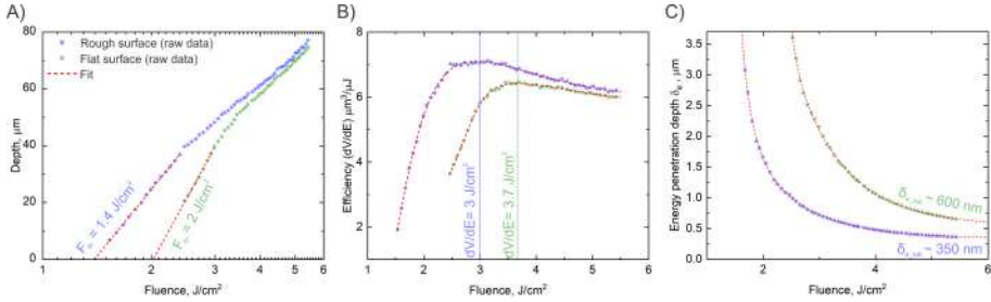
Fig. 4.1 Engraved cavity depth dependence on used laser fluence, when laser processing is applied on flat ( S_{a\_int} < 10 \text{ nm} ) and rough ( S_{a\_int} = 420 \text{ nm} ) surfaces (A). Ablation efficiency ( dV/dE ) dependence on used laser fluence (B). Assessed energy penetration depth \delta_e dependence on used laser fluence. Each cavity measured 0.5 \times 0.5 \text{ mm}^2 is size. The engraving parameters were: laser repetition rate f = 5 \text{ kHz} , scanning pitch dx = dy = 12.3 \text{ μm} , scanning speed v = 61.5 \text{ mm/s} , and included 50 scans per cavity.
