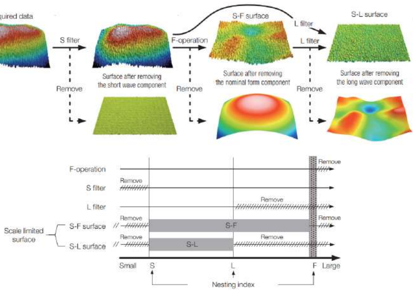
Fig. 1.4 The visual showcase of areal filtration workflow. The upper section of the image illustrates alterations in surface topography resulting from the application of various filters (S, F, and L). The bottom part of the figure shows the filtration operation in the spatial wavelength domain. The S filter is used to remove the shortest wavelengths, the F filter is used for the removal of the form, and finally, the L filter is used for the separation of roughness from waviness.
