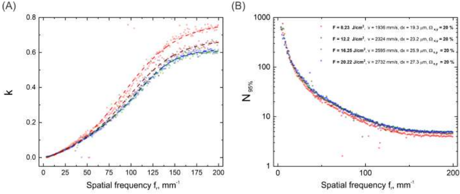
Fig. 5.12 Decay coefficient k dependence on the spatial frequency (A). The number of layers N_{95\%} necessary to reach 95% reduction of the corresponding spatial frequency amplitude (B). Dots represent raw data, while the dashed lines - a visual guide of a trend for the reader. Different colors correspond to different processing parameters. The legend is shared between both figures. The processing was performed on a surface of initial roughness S_{q\_int} = 1.64 \text{ }\mu\text{m} .
