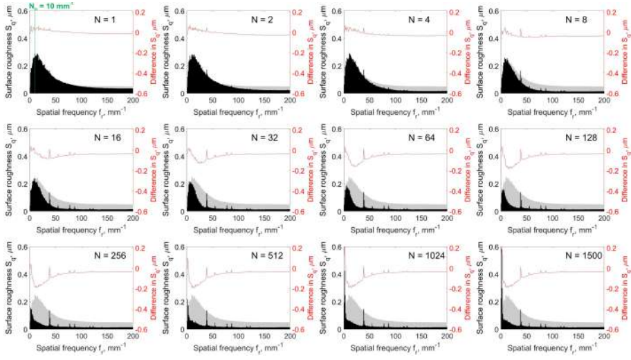
Fig. 5.9 Spatial spectra of surfaces after varying numbers of scans ( N ) are shown in black, while the grey background represents the spectra prior to laser processing. The left y axis indicates the roughness level S_q as a function of spatial frequency. The right y axis displays the change in roughness across spatial frequencies, obtained by comparing the spectra after N scans with that of the unprocessed surface. Processing was performed on a surface with initial roughness of S_{q\_int} = 1.64 \mu\text{m} . Laser processing parameters: fluence F = 16.25 \text{ J/cm}^2 , scanning speed v = 2595.2 \text{ mm/s} , scanning pitch dx = 25.95 \mu\text{m} , overlap of the craters \Omega_{x,y} = 20 \% . The ablation rate under such parameters was R_t = 0.68 \mu\text{m/layer} . The green line indicates the nesting index position that divides the spectra into waviness and roughness parts.
