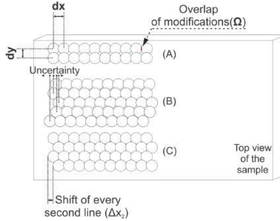
Fig. 3.1 Schematic explanation of different examined scanning strategies. (A) overlap of the craters, (B) uncertainty of first pulse positioning, (C) shift of every second line. dx - distance between single modifications in x direction, dy - distance in y direction, \Omega - overlap of modifications, \Delta x_2 - shift of every second line.
