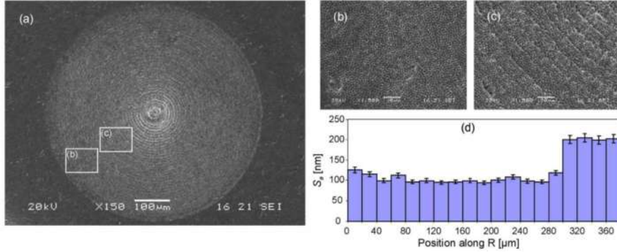
Fig. 1.19 Topography map of a sample machined at E_p = 15 \mu\text{J} , v = 190 \text{ mm/s} . Panel (a) shows the SEM top view of the ablated, panel (b) a magnification of the ablated surface close to the border with the bare surface, panel (c) a magnification at the middle of the ablated layer, panel (d) the variation of the areal roughness S_a measured on 20 \mu\text{m} \times 20 \mu\text{m} square portions of the topography map. The error bars are evaluated on the basis of repeated measurements on different square portions [34].
