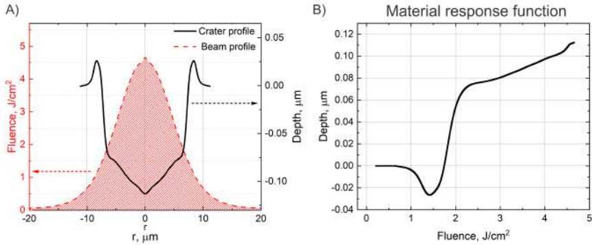
Fig. 3.3 An example of measured and rescaled to its actual size fluence profile of the laser beam at the focal plane and the measured geometry of the crater produced with such laser beam (A). The material response function derived from data in part (A) is given in part (B) of the figure. It shows how much of material is removed at a precise fluence value.
