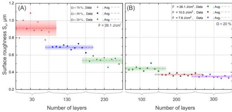
Fig. 4.9 Surface roughness dependence on the number of scans when different scanning algorithms are utilized. Graph (A) shows engraving with different overlaps of the craters, while graph (B) when different pulse energies are used. In both cases, additional scans with different scanning algorithms were scanned on the structures induced by the previous scanning algorithm (see text for clarification). Dots represent raw data, while dashed lines - average values. The extent of the colored area surrounding the average values stands for a range equivalent to one standard deviation. Other processing parameters: \alpha = 73^\circ , \lambda = 1030 \text{ nm} . The uncertainty of layer positioning of a maximum magnitude \Delta \geq dx was maintained.
