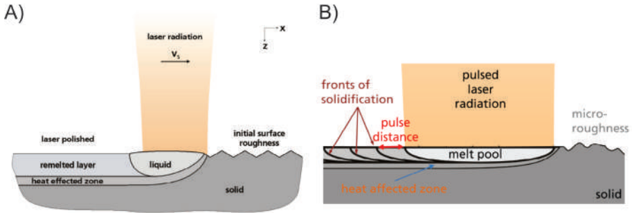
Fig. 7.1 Schematic of laser polishing by remelting a thin surface layer using continuous laser radiation (A) and pulsed laser radiation (B) [26].
