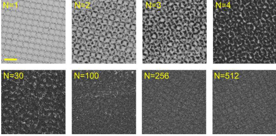
Fig. 5.6 Optical microscope images of laser-processed surfaces after different numbers of scans ( N ). Scale bar is 50 \mu\text{m} . Laser processing parameters: fluence F = 12.2 \text{ J/cm}^2 , scanning speed v = 2324.8 \text{ mm/s} , scanning pitch dx = 23.24 \mu\text{m} , overlap of the craters \Omega_{x,y} = 20 \% .
