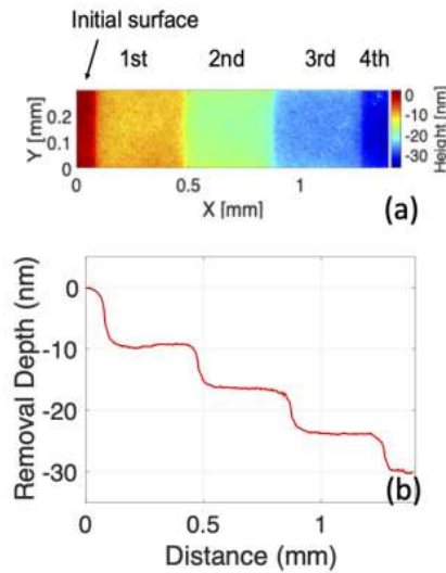
Fig. 7.8 (a) Surface profile of the staircase structure and (b) vertically integrated line profile [231].
