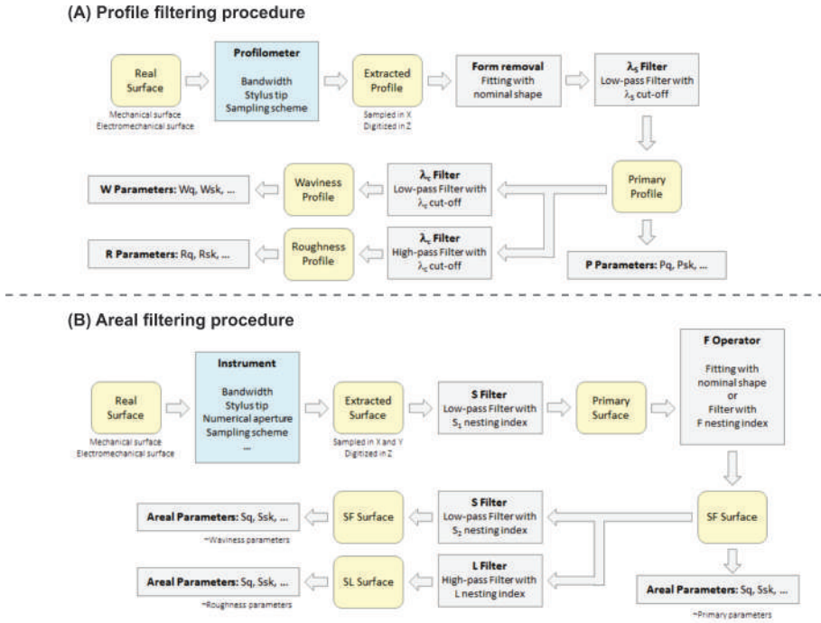
Fig. 1.5 The workflow summarizing the profile (part A) and areal (part B) filtration procedures.
