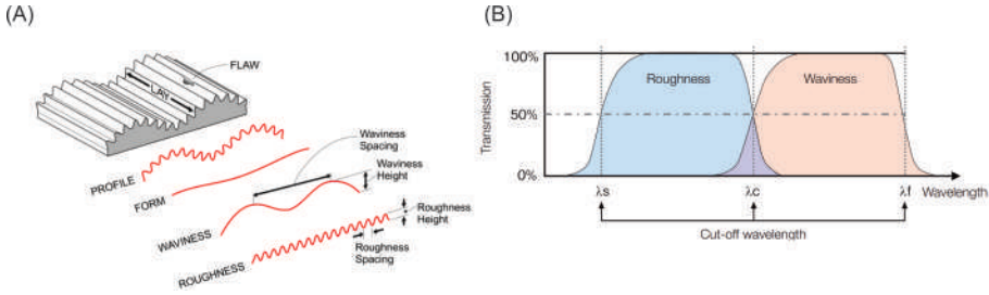
Fig. 1.3 A visual representation depicting that surface texture can be divided into form, waviness, and roughness (A). Filtration operation of the spatial spectrum (B). To obtain roughness cut-offs \lambda_s and \lambda_c are used. To obtain waviness \lambda_c and \lambda_f are used.
