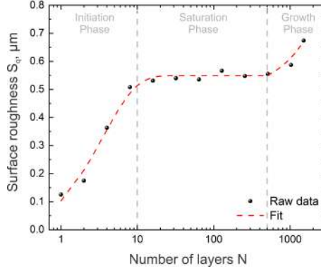
Fig. 5.4 Surface roughness parameter S_q dependence on the number of layers N . Processing was performed on a surface of an optical quality roughness level. Dots show data points, while the dashed line represents the fit. Laser processing parameters: fluence F = 12.2 \text{ J/cm}^2 , scanning speed v = 2324.8 \text{ mm/s} , scanning pitch dx = 23.24 \text{ }\mu\text{m} , overlap of the craters \Omega_{x,y} = 20 \% . The ablation rate under such parameters was R_t = 2.27 \text{ mm}^3/\text{min} ( 0.7 \text{ }\mu\text{m}/\text{layer} ). Spatial spectra of different data points are depicted in figure 5.5.
