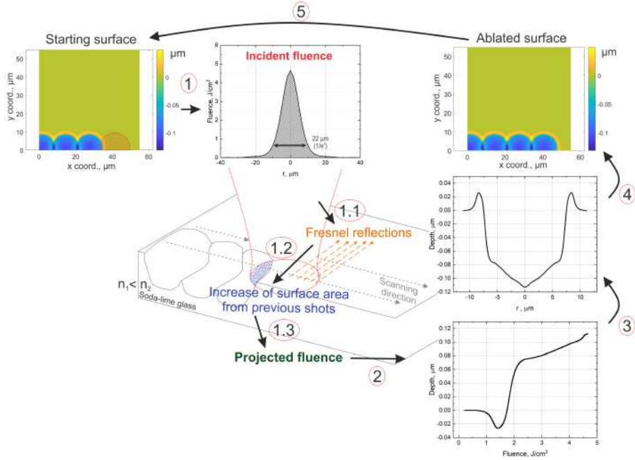
Fig. 3.4 Principle scheme showing the workflow of the numerical model. The incident fluence is projected on the surface (1). Fluence reduction due to fresnel reflections (1.1) and increase of surface area from previous shots (1.2) is taken into account. According to material response function and projected fluence (2) ablated volume is calculated (3). Finally, ablated volume is subtracted from the surface at the current beam location (4). The position of the beam is shifted and calculations are repeated (5).
