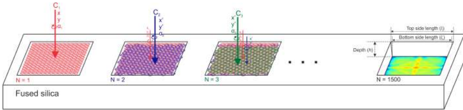
Fig. 6.1 Schematic of the laser engraving process and scanning strategies. Arrows, denoted as c_1 , c_2 and c_3 display the central axis of each layer with corresponding spatial coordinates x , y and angle of rotation \alpha_n . Different colors stand for different layers. N stands for number of scans performed on the surface.
