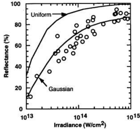
Fig. 1.10 Reflectivity of fused silica as a function of laser irradiance for \lambda = 1053 nm and \tau_p = 350 fs. Calculations of R values for two cases are given when laser beam has a uniform and gaussian intensity distributions. Governing equations are given in ref. [114].
