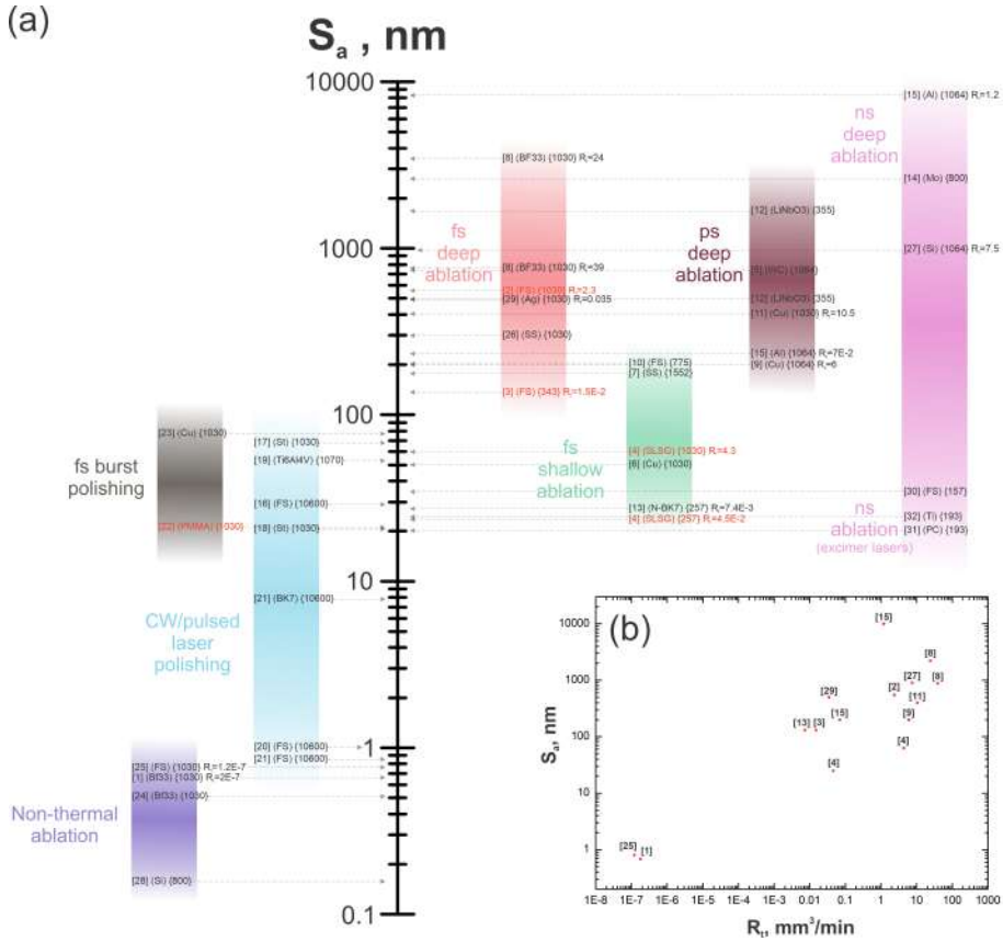
Fig. 7.9 Part (a) of the figure overviews the attainable surface roughness ( S_a ) levels when different laser processing techniques are used. Next to the reference from which the value is taken, additionally the processed material abbreviation, together with laser radiation wavelength (in nm) and ablation rate (in mm 3 /min units), when available, are given. Red references correspond to the results achieved in this work. The part (b) of the figure plots the S_a dependence on material removal rate R_t from the references containing both values. 1 - [231]; 2 - [237]; 3 - [36]; 4 - [66]; 5 - [35]; 6 - [172]; 7 - [34]; 8 - [33]; 9 - [162]; 10 - [160]; 11 - [156]; 12 - [154]; 13 - [152]; 14 - [148]; 15 - [147]; 16 - [10]; 17 - [217]; 18 - [26]; 19 - [218]; 20 - [221]; 21 - [222]; 22 - [25]; 23 - [238]; 24 - [233]; 25 - [236]; 26 - [170]; 27 - [165]; 28 - [239]; 29 - [240]; 30 - [241]; 31 - [242]; 32 - [224]. FS- fused silica; SLSG - soda lime; BF33 - borofloat33; WC- tungsten carbide; Cu -copper; SS - stainless steel; Mo - Molybdenum; Al - Aluminum; St - steel; PMMA - hydrophilic acrylic polymer, Ag - silver, Ti - titanium, PC- polycarbonate.
