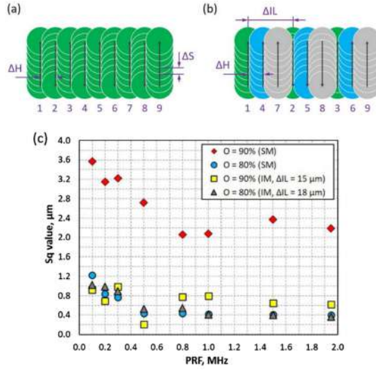
Fig. 1.18 Illustration of bi-directional: (a) sequential and (b) interlaced laser beam scanning methods. Symbols: \Delta H – hatch distance, \Delta S – pulse-to-pulse distance along the linear movement of the laser beam, and \Delta IL – interlacing distance. Part (c) of the figure depicts the surface roughness ( S_q ) dependence on laser pulse repetition frequency (PRF) when different overlap values ( O ) and different scanning strategies are utilized [33].
