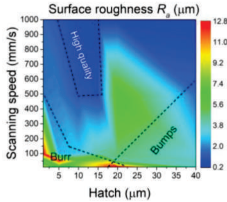
Fig. 1.17 The surface roughness of the bottoms of the cavities after one scan dependence on scanning speed and hatch distance with quality regions [162].
