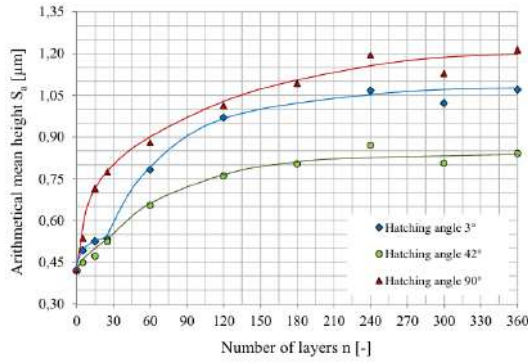
Fig. 1.22 Evolution of surface roughness, when different hatching angles are used [35].
