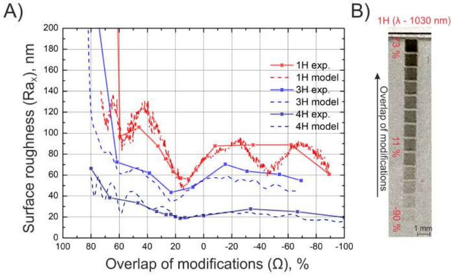
Fig. 3.6 Surface roughness dependence on the overlap of modifications, when different laser wavelengths are used (A). Surface roughness measured in scanning (x) direction. Solid lines represent experimental results, and dotted - modeling results. In part B, a macro picture of machined surfaces with \lambda = 1030 nm (1H) is shown. Pulse energies used: for 1H - E_p = 173 \mu\text{J} , for 3H - E_p = 10.8 \mu\text{J} and for 4H - E_p = 8.72 \mu\text{J} .
