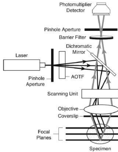
Fig. 1.6 The main components of a modern laser scanning confocal microscope. Light from one or more lasers passes through a pinhole, is attenuated through an AOTF (acoustic-optic tunable filter), bounces off a dichromatic mirror, and passes into the scanning unit. A scanned beam enters the back focal plane of the objective lens, which focuses the light at a point in the specimen. The reflected light undergoes filtration through a pinhole aperture to exclusively transmit the light gathered from the focal plane, which is then detected by a photomultiplier detector [86].
