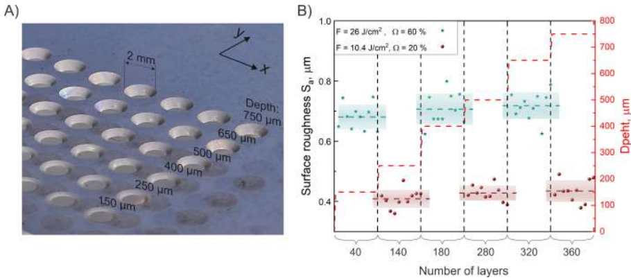
Fig. 4.10 (A) A photo of the sample after deep-engraving. In the y direction cavities of different depths can be seen, whereas in the x direction, cavities ablated using identical parameter sets are shown. In part (B) of the figure, surface roughness and depth of the cavity dependencies on the number of scans are presented. Dots represent raw data, while dashed lines - averaged values. The extent of the colored area surrounding the average values represents the range equal to one standard deviation. Other processing parameters: \alpha = 73^\circ , \lambda = 1030 nm. The uncertainty of layer positioning of a maximum magnitude \Delta \geq dx was maintained.
