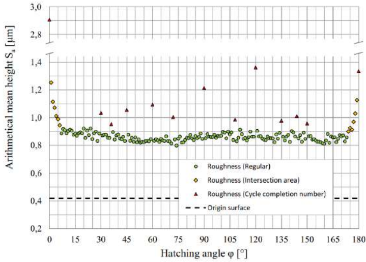
Fig. 1.21 Surface roughness dependence on hatching angle, when the surface is scanned 360 times [35].
