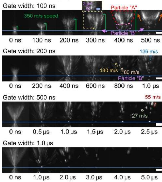
Fig. 1.12 Scattering images showing the ablation dynamics at a fluence of 18.7 \text{ J/cm}^2 and pulse duration of 500 fs, across different time scales. Scattering images were acquired for varying ICCD gate widths of 100 ns, 200 ns, 500 ns, and 1 \mu\text{s} , respectively. The blue lines in these images represent the Cu target surface, and images below the lines are mirror reflections from the polished Cu surface. White scale bars, 50 \mu\text{m} [123].
