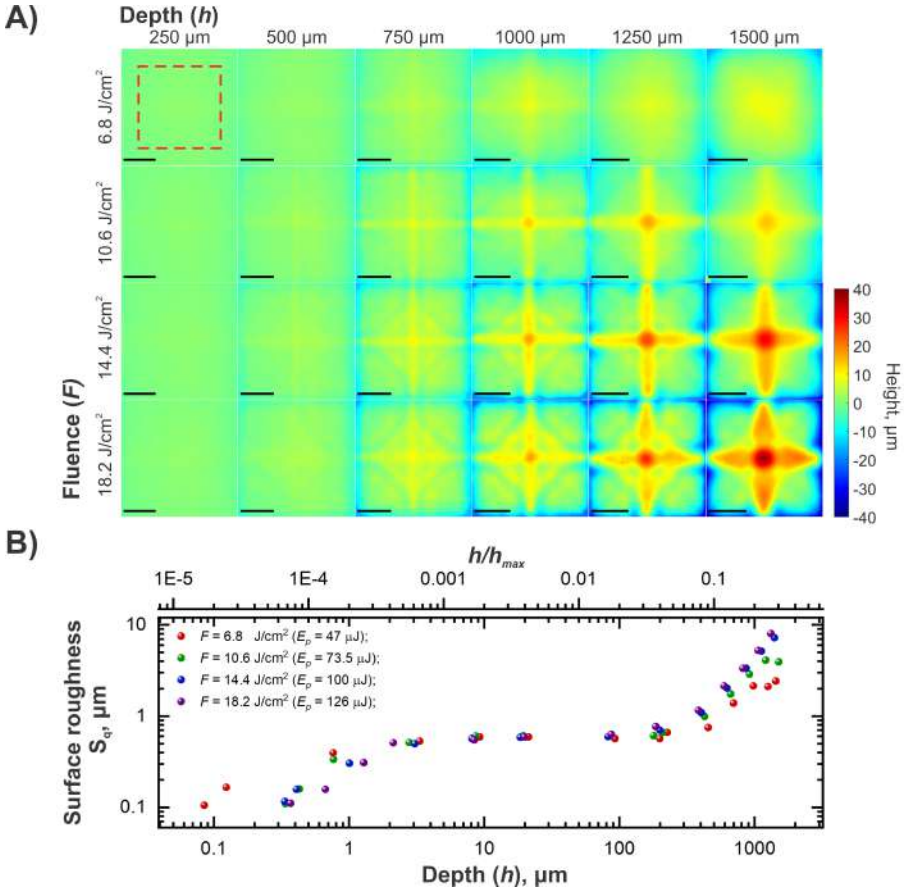
Fig. 6.2 Height maps of the bottom surfaces of deep ablated rectangular cavities of varying depths produced using different fluences F (A). Surface roughness parameter S_q dependence on the engraved depth, when different F values are used (B). The top x axis shows engraved depth normalized to the sample thickness h_{\text{max}} (5 mm). Other laser parameters were fixed: scanning speed v = 2325 mm/s, scanning pitch dy = dx = 23.3 \mu\text{m} . The black bar indicates a length of 1 mm, the red dashed rectangle shows the area from which the roughness was calculated (representing 2.1 mm x 2.1 mm in size).
