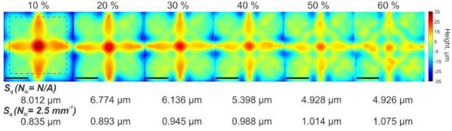
Fig. 6.5 Height maps of the bottom surfaces of deep ablated rectangular cavities obtained using different crater overlap values \Omega . For each surface, the S_q values estimated from a 2.5 \times 2.5 \text{ mm}^2 rectangular area (indicated by the red dashed rectangle) are reported for both the unfiltered case ( N_{ic} = N/A ) and after eliminating low spatial frequencies ( N_{ic} = 2.5 \text{ mm}^2 ). Laser processing parameters used: fluence F = 18.2 \text{ J/cm}^2 , scanning speed v , line pitch dy and number of scans N were varied to reach an engraved depth of h \approx 1000 \mu\text{m} . The black bar indicates a length of 1 mm.
