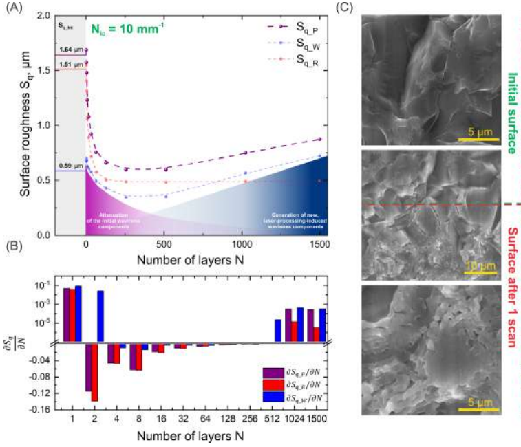
Fig. 5.11 Surface roughness S_q dependance on the number of layers scanned N (A). The S_q values associated with the waviness and roughness parts of the surface texture are denoted as S_{q-W} , S_{q-R} respectively, while the S_q value of the entire surface texture is indicated as S_{q-P} . Variation of the local derivatives \partial S_{p,r,w}/\partial N as a function of the number of layers N (B). SEM images of initial surface texture (initial roughness of S_{q-int} = 1.64 \mu\text{m} ) and surface texture after a single scan (C). Laser processing parameters: fluence F = 16.25 \text{ J/cm}^2 , scanning speed v = 2595.2 \text{ mm/s} , scanning pitch dx = 25.95 \mu\text{m} , overlap of the craters \Omega_{x,y} = 20 \% . The nesting index used to separate waviness and roughness components was set to N_{ic} = 10 \text{ mm}^{-1} .
