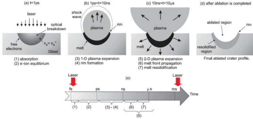
Fig. 1.11 A schematic description of ablation process of glass with a femtosecond laser pulse (a)–(d) and time scales associated with various processes (e) [119].
