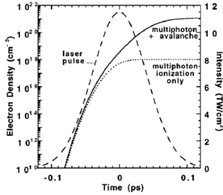
Fig. 1.9 Total (solid) and multiphoton produced (dotted) electron densities are plotted along with the Gaussian pulse shape. Seed electrons are produced by multiphoton ionization at the pulse peak after which an avalanche produces a critical density [111].
