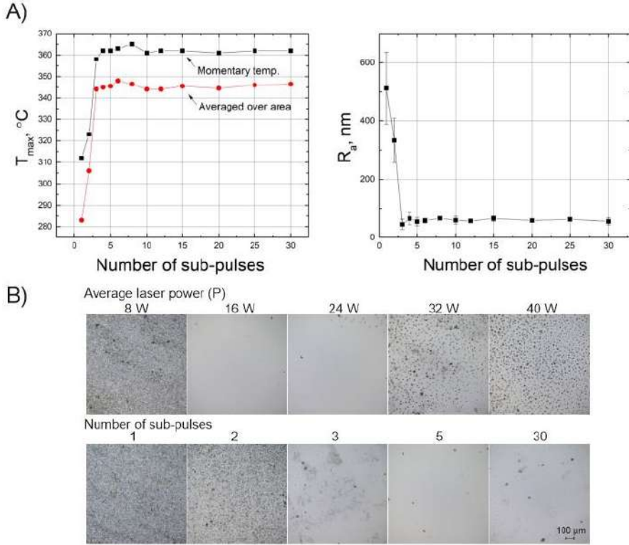
Fig. 7.6 (A) Surface temperature dependence on the number of sub-pulses within a burst (on the left), R_a dependence on the number of sub-pulses within a burst (on the right). Other parameters: P = 16 \text{ W} , dy = 10 \mu\text{m} , v = 700 \text{ mm/s} and number of scans = 2. (B) The microscope pictures of laser polished surfaces using different P values, with the remaining parameters of N_p = 10 , dy = 10 \mu\text{m} , v = 700 \text{ mm/s} and number of scans = 2 (upper row). The microscope pictures of laser polished surfaces using different numbers of sub-pulses. Remaining parameters P = 16 \text{ W} , dy = 10 \mu\text{m} , v = 700 \text{ mm/s} and number of scans = 2 (bottom row).
