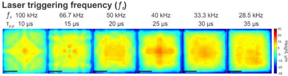
Fig. 6.4 Height maps of the bottom surfaces of deep ablated rectangular cavities, when scanning is performed under identical conditions, with only varying parameter being the pulse repetition period \tau_{p-p} . Laser processing parameters used: fluence F = 18.2 \text{ J/cm}^2 , overlap of the craters \Omega = 20 \% , number of scans N = 775 , engraved depth h = 820 \mu\text{m} . The black bar indicates a length of 1 mm.
