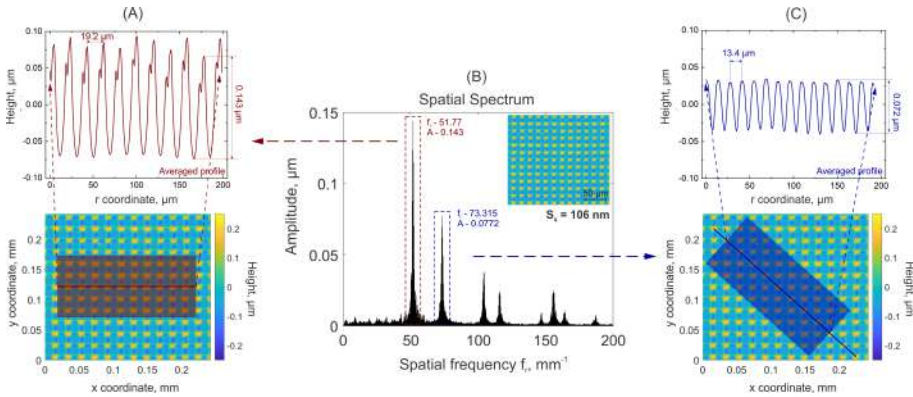
Fig. 5.3 A horizontal profile averaged over red-colored area (A). Spatial spectrum of a single-scanned surface (B). A diagonal profile averaged over blue-colored area (C). Laser processing parameters: fluence F = 8.23 J/cm 2 , scanning speed v = 1937 mm/s, scanning pitch dx = 19.36 μm.
