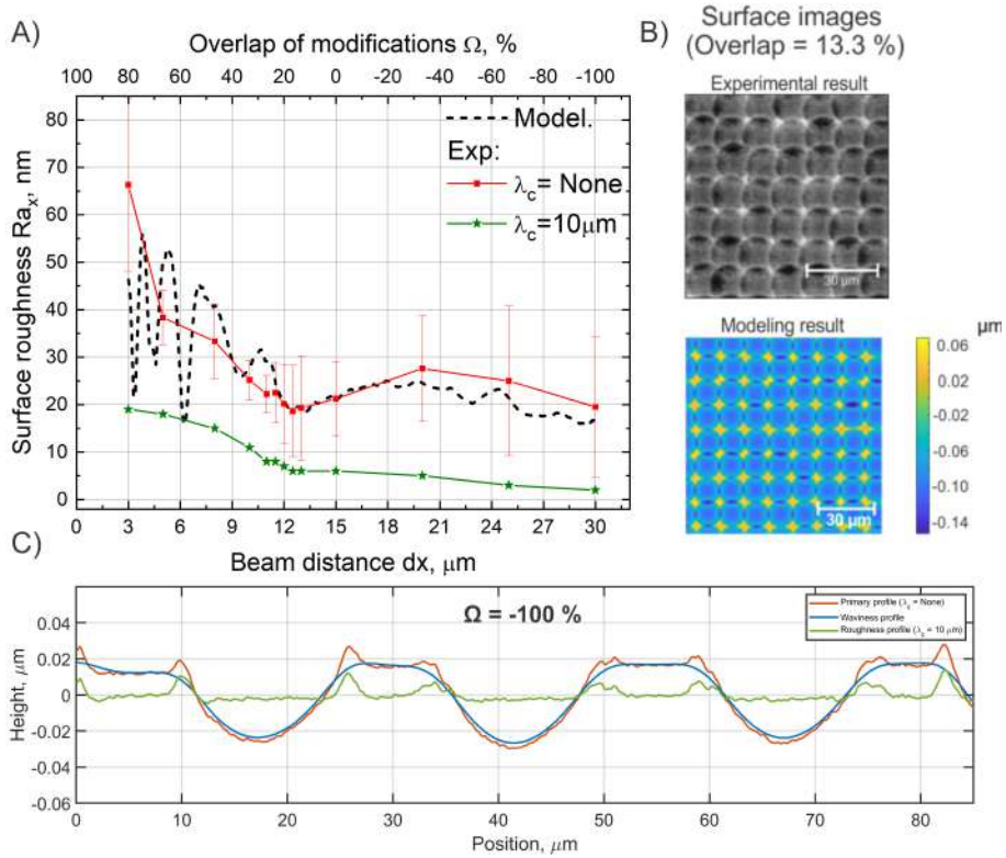
Fig. 3.5 Surface roughness (in the scanning direction) dependence on the overlap of modifications (A). The black dashed line represents the numerical modeling results, whereas the red and green curves correspond to the experimental results obtained without filtering and with a cutoff wavelength of \lambda_c = 10 \mu\text{m} , respectively. Surface images after single-pass machining acquired experimentally and via numerical calculations (numerical model description given in section 3.2) when the overlap of modifications is 13.3 % (B). Part (C) compares the surface profiles obtained without a \lambda_c filter (red) and with a cutoff wavelength of \lambda_c = 10 \mu\text{m} (green). The experiments were performed with 3^{rd} experimental setup configuration and E_p of 8.72 \mu\text{J} .
