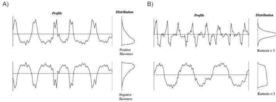
Fig. 1.1 The visual representation of roughness parameters skewness and kurtosis. Part (A) depicts the skewness roughness parameter. The upper profile represents a case when R_{sk} > 0 , and the lower one a case when R_{sk} < 0 . Part (B) shows the roughness parameter - kurtosis. The upper profile depicts a case when the profile is leptokurtic ( R_{ku} > 3 ), whereas in the bottom part, a platykurtic case is shown ( R_{ku} < 3 ) [68].
