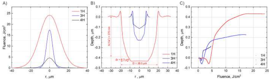
Fig. 3.7 Beam profiles for different laser wavelengths (A), cross-sectional profiles of single-shot modifications in soda-lime glass induced by different wavelengths (B), and material response functions corresponding to the various wavelengths (C). Red curve - 1H ( E_p = 173 \mu\text{J} ; F = 24 \text{ J/cm}^2 ), blue curve - 3H ( E_p = 10.8 \mu\text{J} ; F = 17.3 \text{ J/cm}^2 ), black curve - 4H ( E_p = 8.72 \mu\text{J} ; F = 4.6 \text{ J/cm}^2 ).
