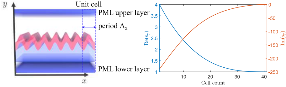
Figure 1.9: PML of a device with PBCs (a) and the unit cell (b) with transverse periodicity.
