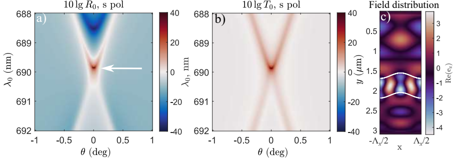
Figure 5.3: Reflection (a,d) and transmission (b,e) spectra with the respective guided resonant modes (c,f) of sup-wavelength operating regime. The arrow indicates field the spectral location for field distribution.
