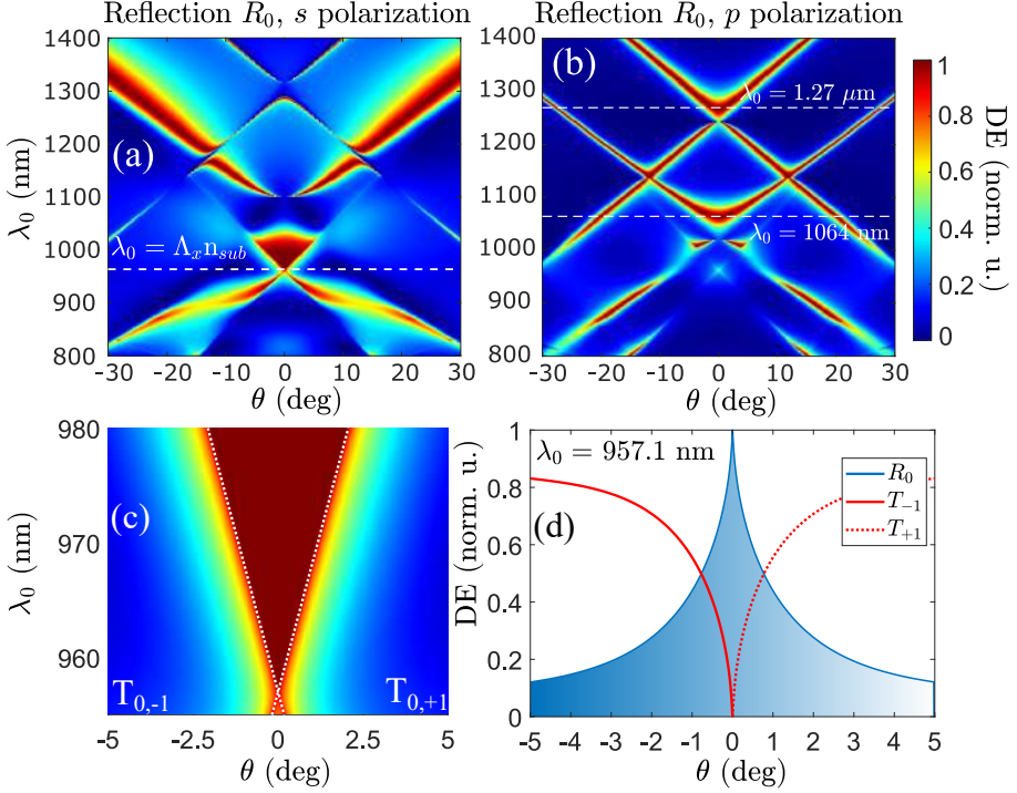
Figure 2.4: Zeroth order reflection of s polarization (a,c) and p polarization (b), alongside with diffraction efficiencies (d) for s polarized input. Dashed lines (and red ones) refer to additional diffraction orders.
