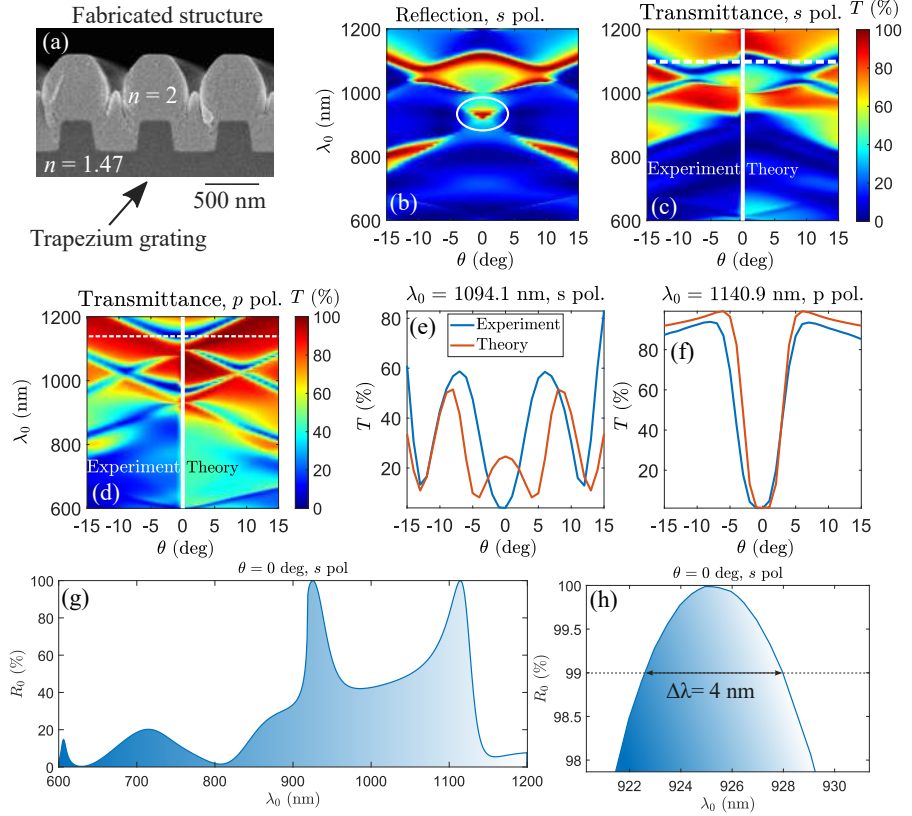
Figure 2.5: Cross-section of the fabricated structure (a), Simulated zeroth order reflection spectrum (b) with triangular reflection, zeroth order transmission comparison between measured and simulated maps of s (c) and p (d) polarizations, as well as their angular profiles in (e) and (f), respectively. The computed reflectance spectrum at normal incidence (g) and its zoom at (h).
