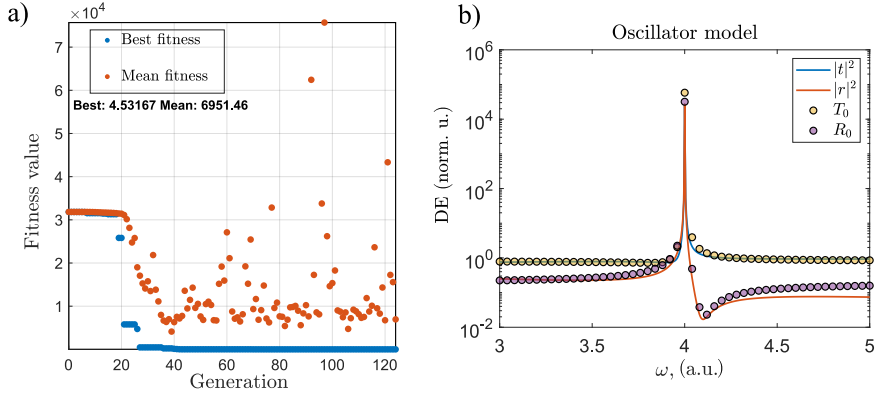
Figure 5.9: Optimization results (a) for the presented parameters in Table 5.4. The oscillator analytical model's comparison with the model's results, illustrated in Fig. 5.5 (a). The dots in the graph (b) represent numerically computed zeroth order diffraction efficiencies, whereas the lines represent resonance fitting.
