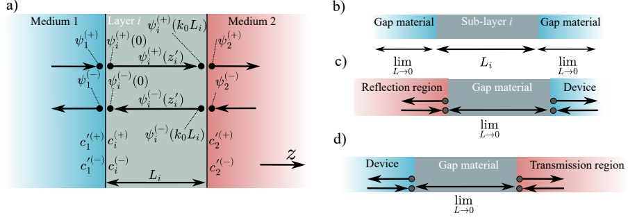
Figure 1.15: Schematics for S matrix method, involving asymmetrical layout of media between intermediate layer i (a), symmetrical layout of vacuum layers between intermediate sub-layer (b), and schematics for computation S matrix of reflection (c) and transmission (d) regions.
