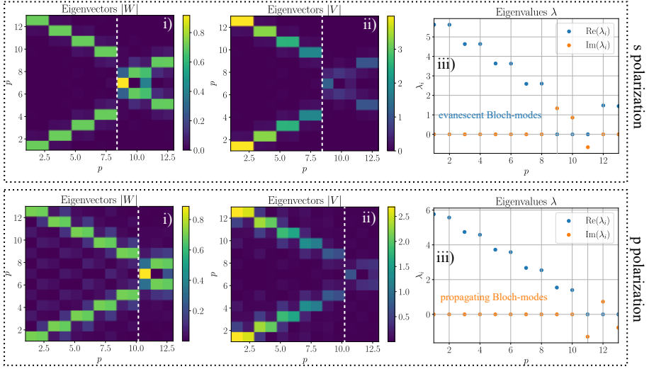
Figure 1.14: 2D RCWA eigen-vector (i,ii) and eigenvalue (iii) visualization of a rectangular grating, whose filling factor f = 0.5 , n_{1,2} = [1.47, 1] , transverse periodicity \Lambda_x = 0.6 \mu\text{m} , \lambda_0 = 0.6 \mu\text{m} , \theta = 0 \text{ deg} .
