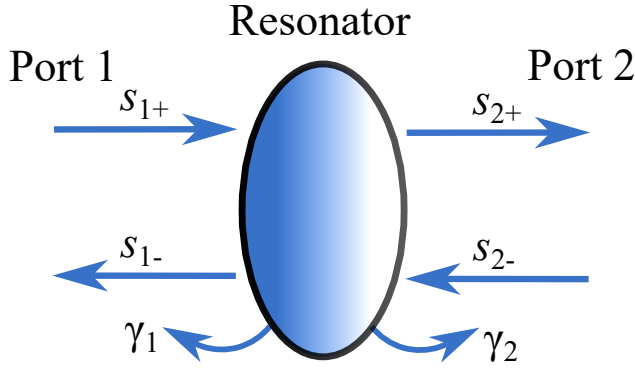
Figure 1.5: TCMT's concept of a resonator with 2 ports with decay coefficients \gamma_1 and \gamma_2 .
