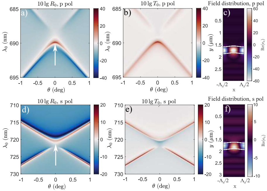
Figure 5.4: The enlarged reflection (a,d) and transmission (b,e) spectra with the respective guided resonant modes (c,f) of sub-wavelength operating regime.
