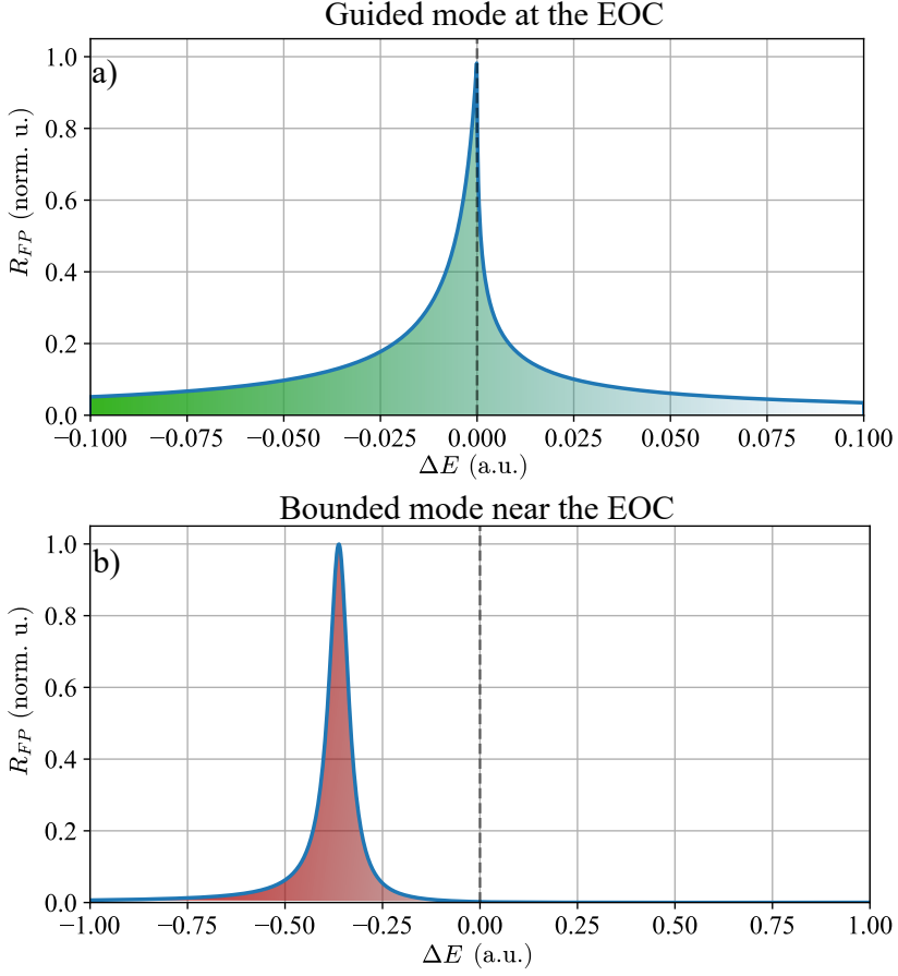
Figure 3.2: Two resonance types encountered in FP potential well model - An asymmetrical resonant reflection at the EOC (a), derived from Eq. (3.17) and bounded mode near the EOC (b), achieved from Eq. (3.16). The parameters chosen here are as follows: a = \pi/2 , t = 0.6 , \gamma_0 = 0.16 , V = 2 .
