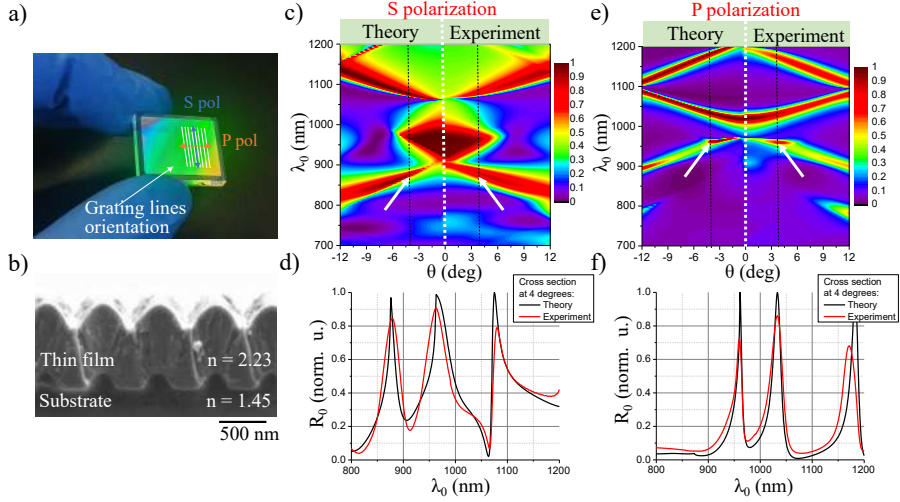
Figure 3.4: Photo of fabricated GMR filter (arrows indicate polarization directions (a), and the SEM image of specimen sample cross-section (b). Numerical/measured spectra of the reflection in the plane of angle-wavelength for (c,d) S polarization and (e,f) P polarization, with their cross-sections at 4 degrees of light incidence angle. The arrows indicate guided modes crossing the EOC.
