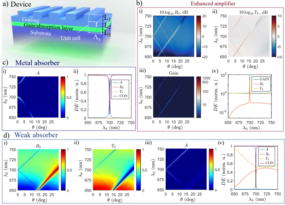
Figure 6.6: DFB system which utilizes GMR-based coupling from the grating with gain/absorption layer (a). The enhanced gain spectrum is shown in b), given the Diffraction Efficiencies (DE) R_0 and T_0 , as well as values for normal incidence (shown in b, iv). The absorption A profiles of the metallic absorber are shown in c). The weak absorber's DE characteristics are provided in d).
