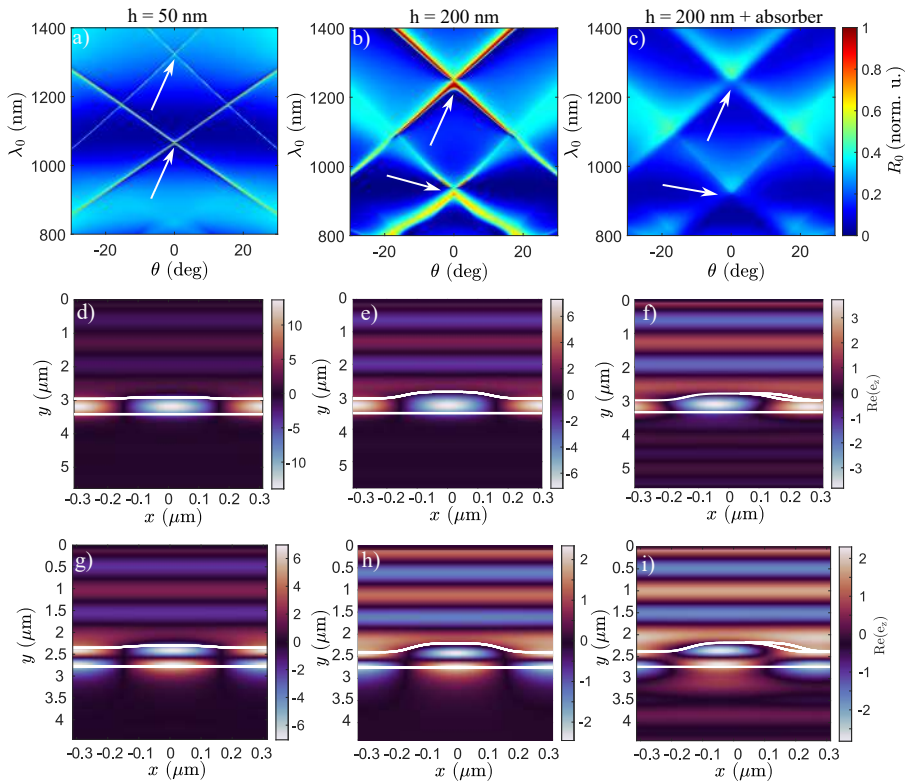
Figure 4.3: Numerically calculated reflectance map for s polarization of TiO 2 layer on silica substrate. Small amplitude periodic perturbation is represented in (a) with its first (d) and second (g) order guided modes. The strong periodic perturbation (b) and respective field configurations (e,h) as well as with the absorber (c) with the respective field configurations (f,i),
