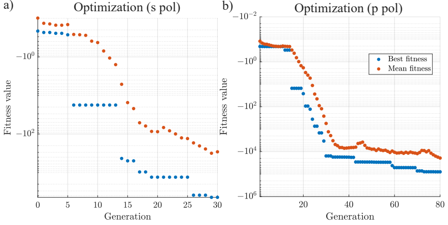
Figure 5.2: The genetic algorithm's optimization procedure for s polarization a) and for p polarization b).
