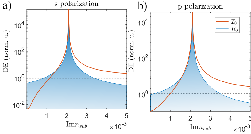
Figure 5.6: The dependence of zeroth order diffraction efficiencies from imaginary part of the refractive index of thin film for s polarization a) and p polarization b) at normal incidence.
