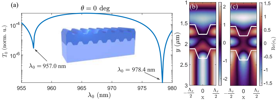
Figure 2.3: Zeroth order transmission with its spectral dips (a) and field distributions given those dips (b,c). The fields (b) and (c) correspond to the transmission dips at \lambda_0 = 957.0 nm and \lambda_0 = 978.4 nm.
