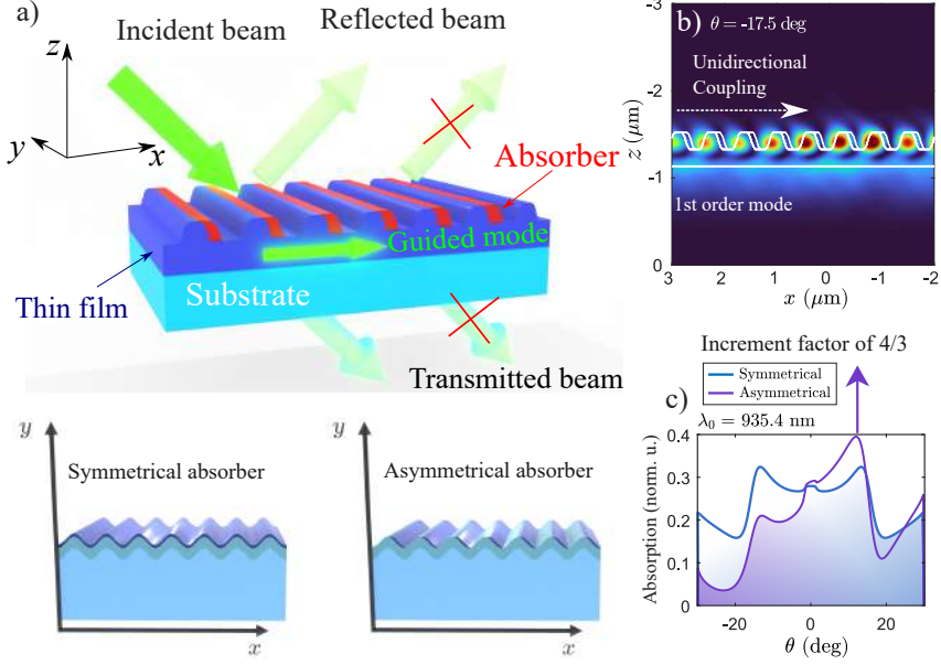
Figure 4.1: Absorption enhancement concept (a), first order GMR mode (b) and comparison between symmetrical and asymmetrical absorptions (c), resulting in increment of absorption.
