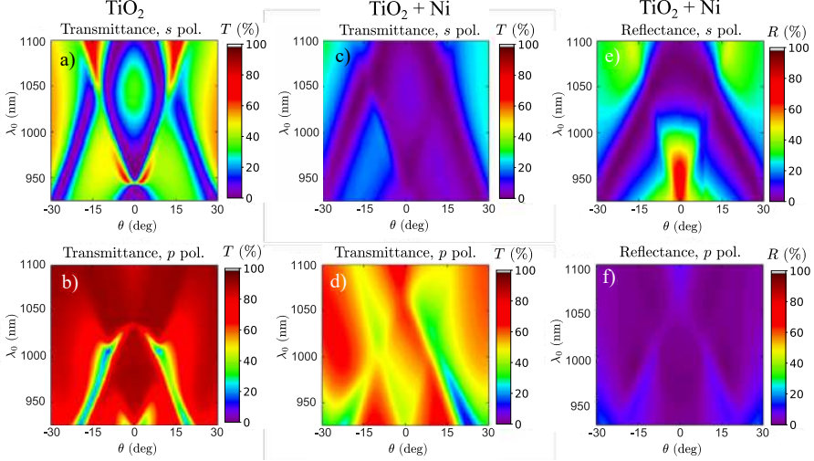
Figure 4.6: Experimentally measured zeroth order transmission spectrum of s and p polarization for L = 300 nm GMR \text{TiO}_2 thin film filter without absorber (a,b). The zeroth order diffraction efficiency measurements for asymmetrically placed absorber is present for s (transmittance c) and reflectance e)) and p polarizations (transmittance d) and reflectance f)).
