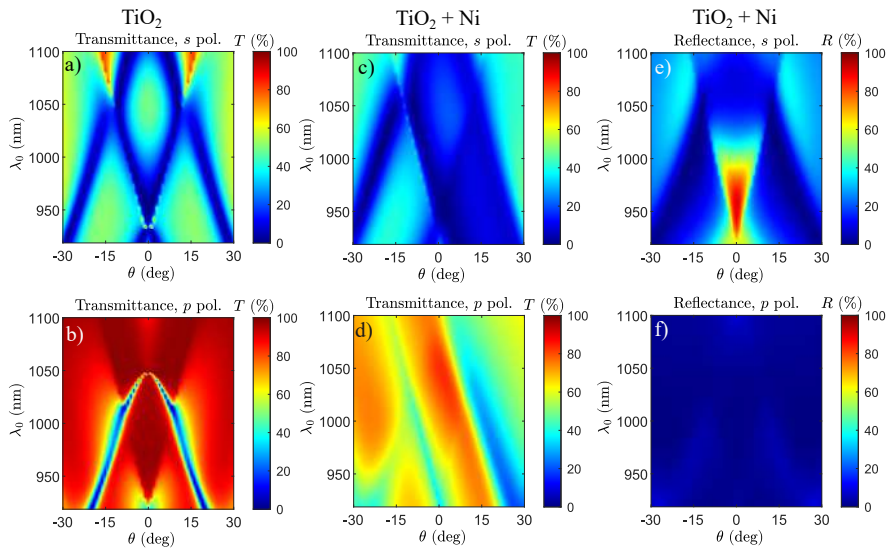
Figure 4.5: Numerically simulated zeroth order transmission spectrum of s and p polarization for L = 300 nm GMR \text{TiO}_2 thin film filter without absorber (a,b). The zeroth order diffraction efficiency maps for asymmetrically placed absorber is present for s (transmittance c) and reflectance e)) and p polarizations (transmittance d) and reflectance f)).
