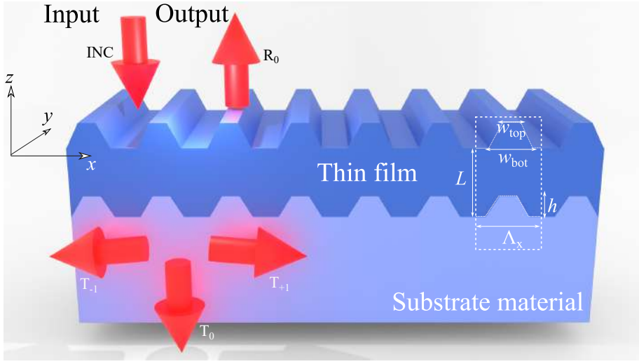
Figure 2.1: The angular filtering device with double periodic thin film modulation via trapezium interface.
