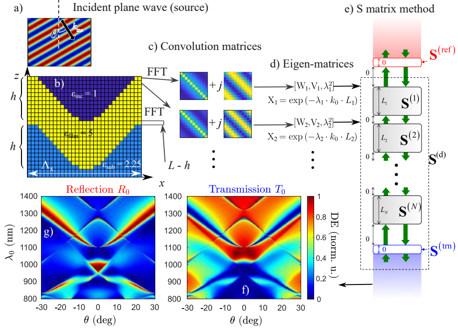
Figure 1.16: A conceptual schematic of RCWA algorithm with memory efficient Scattering matrix method. The step-wise parts are presented in the following: a) incident source field as a plane wave, b) transversely periodic discrete GMR filter/coupler, c) Toeplitz matrices of Fourier transformed sub-layers, d) Eigen-matrices of \Omega matrix e) S matrix method schematic (block connection, adapted from [92]) and f) and g) are zeroth order transmission and reflection values of the device b).
