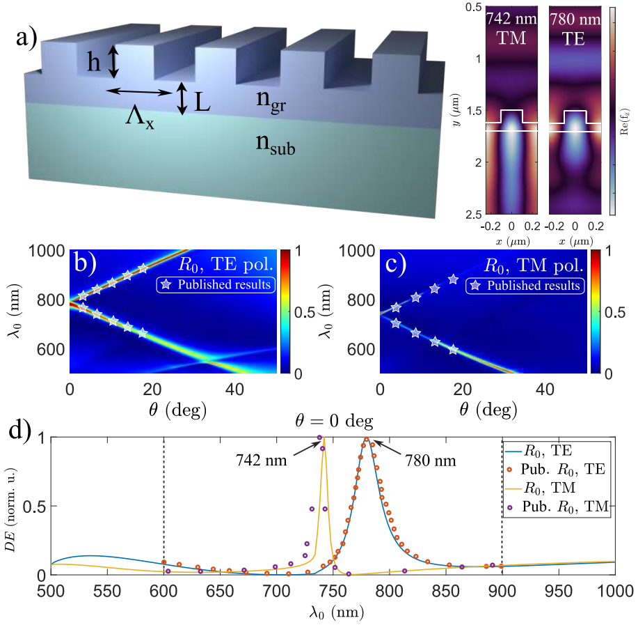
Figure 6.2: Guided mode resonance reflection spectra of SiN 4 grating via the RCWA approach. Accordingly, (a) for TE (b) and TM (c) polarizations, as well as diffraction efficiencies for both polarizations at normal incidence (d). The structure is derived from [147]. The dotted line in d)
