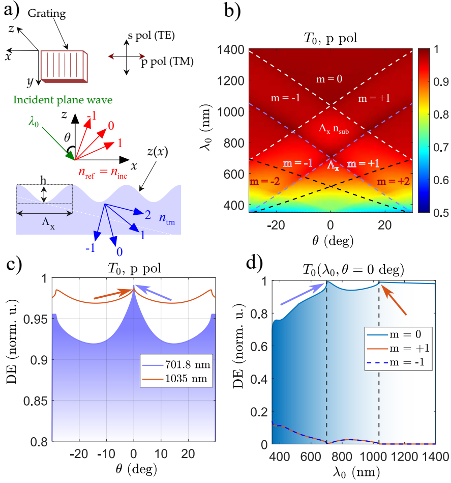
Figure 1.3: Visualization of Rayleigh anomaly given the harmonic grating (a), transmission spectrum for p polarization at (b), angular dependence (c) and transmission dependency at normal incidence (d). The grating parameters are: n_{\text{sup}} = 1, n_{\text{sub}} = 1.48, h = 0.2 \mu\text{m}, \Lambda_x = 0.7 \mu\text{m} . Simulations are performed with 2D RCWA. Light-purple arrows indicate \lambda_R for which R_{\pm 1} orders appear/disappear, orange arrows indicate sudden diffraction order T_{\pm 1} appearance/disappearance in (c) and (d).
