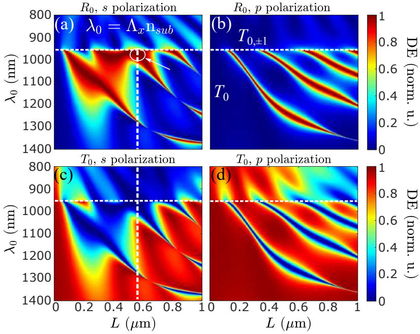
Figure 2.2: Zeroth order reflection profiles for s polarization (a) and p polarization (b) and the transmittance spectra for respective polarizations in (c) and (d). Angle of incidence is \theta = 0 deg.
