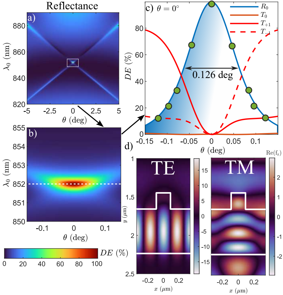
Figure 6.4: Magnusson's spatial filtering results first reported in [86] and reproduced here with "ZenScat". The zeroth order reflection is denoted at a) zoomed at b), the diffraction efficiency is present at with benchmark data represented with green dots c) for the thin film GMR sup-wavelength grating, shown at d).
