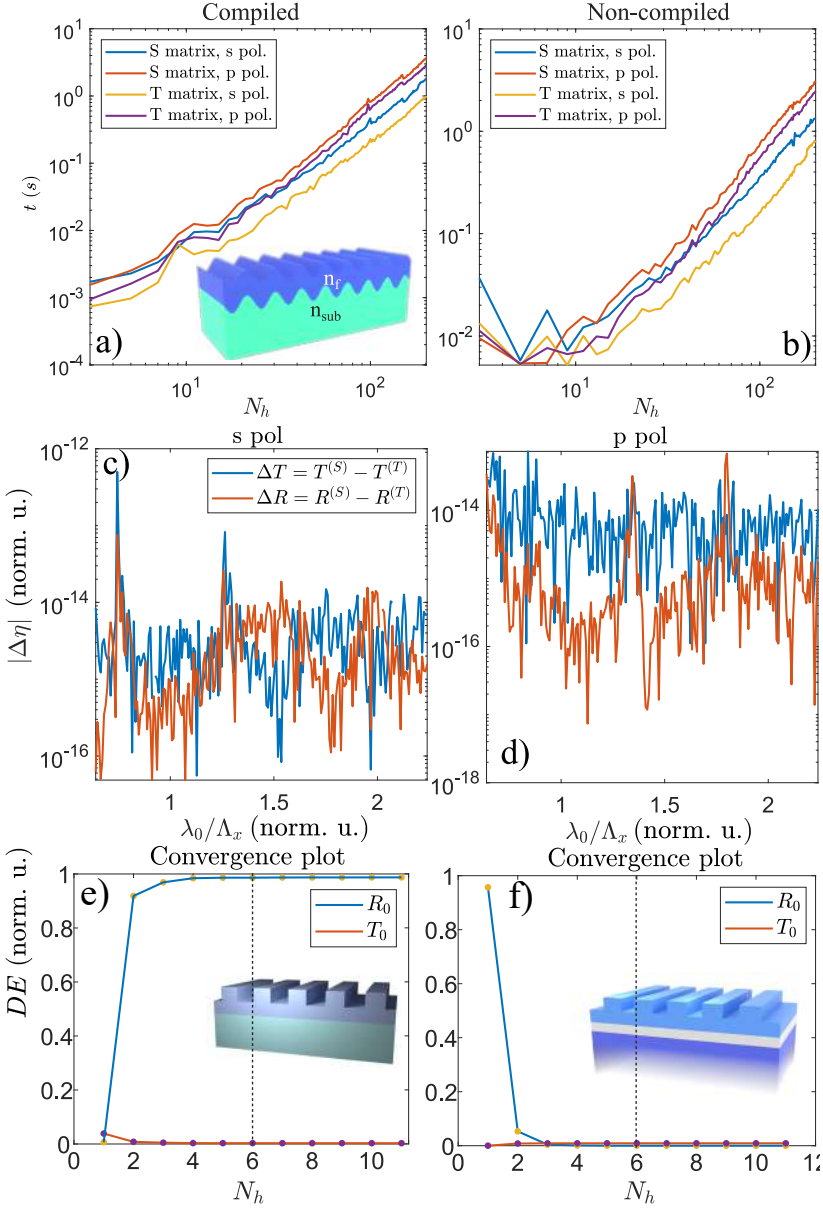
Figure 6.7: Algorithm performance with compiled (a) and non-compiled (b) matrix methods. The diffraction efficiency errors for monolayered GMR filter for s and p polarizations (c,d) for \theta = 15 deg angle of incidence. The convergence results are for rectangular GMR filter [147] e) and metallic DFB device from optimization case (f).
