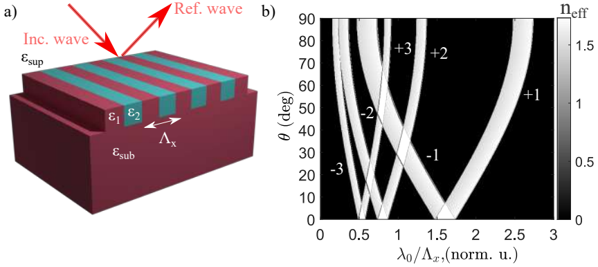
Figure 1.4: The Schematic of GMR and its location in wavelength/angular domain, adapted from [79] in a) and GMR distribution in a harmonic interfaced thin-film waveguide b).
