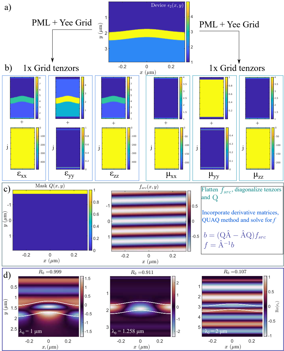
Figure 1.12: 2D FDFD schematic for calculating light scattering by enforcing PBC in transverse ( x ) and PML in propagation ( y ) directions.
