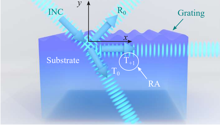
Figure 1.2: The schematic of the Rayleigh anomaly (RA) concept - incident wave (INC) is at an oblique angle, which is then reflected and transmitted via the grating and Rayleigh anomaly corresponds to the longitudinally propagating wave along the surface of the grating. In this case, it is T_{+1} diffraction order.
