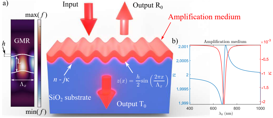
Figure 5.1: The concept of a GMR filter with active thin film a), enhancing diffraction efficiencies. Anomalous dispersion cases of b) amplification, used in this section.
