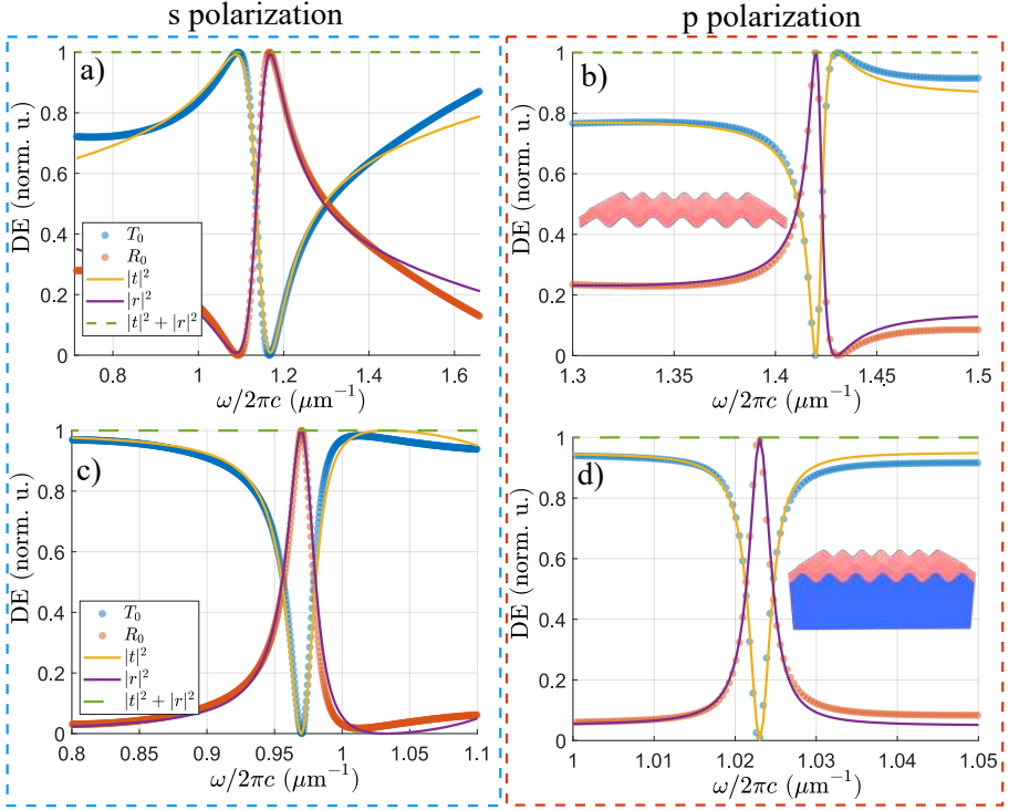
Figure 1.6: Curve fitting representation of the GMRs for a single symmetrical harmonic layer in the air (a,b) and a filter with FS substrate (c,d).
