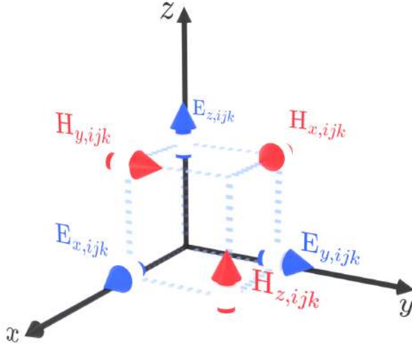
Figure 1.10: A representation of a rectangular 3D cell of the Yee grid.
