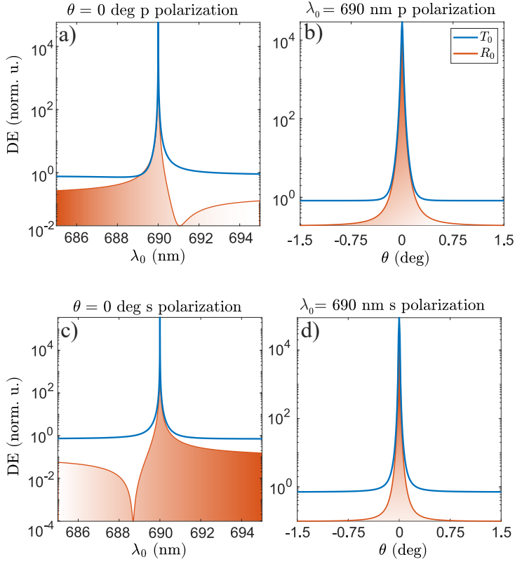
Figure 5.5: The zeroth order diffraction efficiencies at normal incidence (a,c) for p and s polarizations, as well as their angular dependence at peak gain (b,d).
