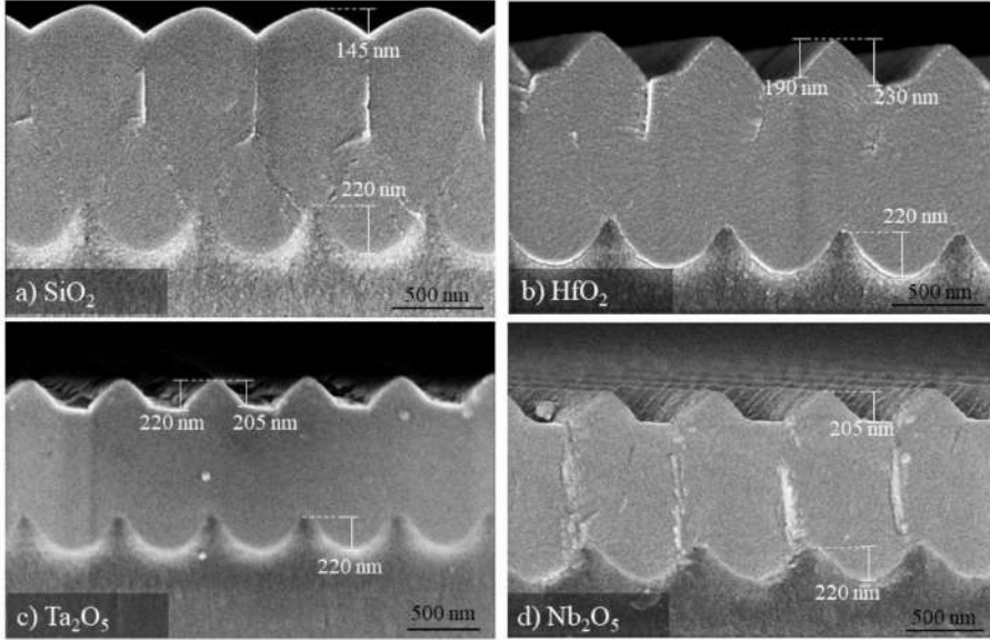
Figure 1.8: The surface replication study by deposition of various oxides via IBS method, adapted from [87]. The top oxide layers with their respective refractive indexes at 970 nm are ordered in the following: \text{SiO}_2 , n = 1.48 a), \text{HfO}_2 , n = 1.99 b), \text{Ta}_2\text{O}_5 , n = 2.09 c), \text{Nb}_2\text{O}_5 , n = 2.25 d). Scanning Electron Microscope (SEM) is used to visualize fabricated sample slices.
