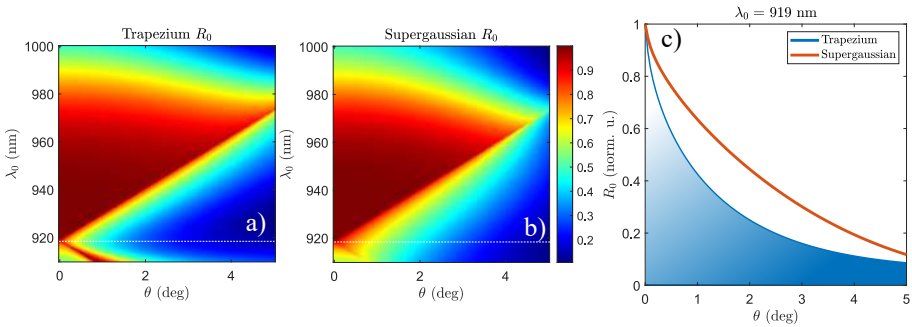
Figure 3.5: Computed zeroth order reflection spectra for trapezium (a) and supergaussian (b) thin film broadband filters, which and the reflectance slice at \lambda_0 = 919 nm (c), which is marked by a plotted white line in (a) and (b).
