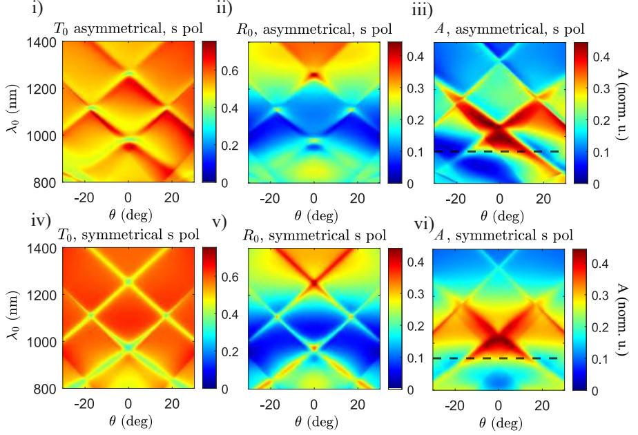
Figure 4.2: The calculated spectra for asymmetrical (i - iii) and symmetrical (iv-vi) device's zeroth order transmission, reflection and absorbance (given flat interface function). The dashed lines are at 935.4 nm, used for absorption comparison, which is visualized in Fig. 4.1 c).
