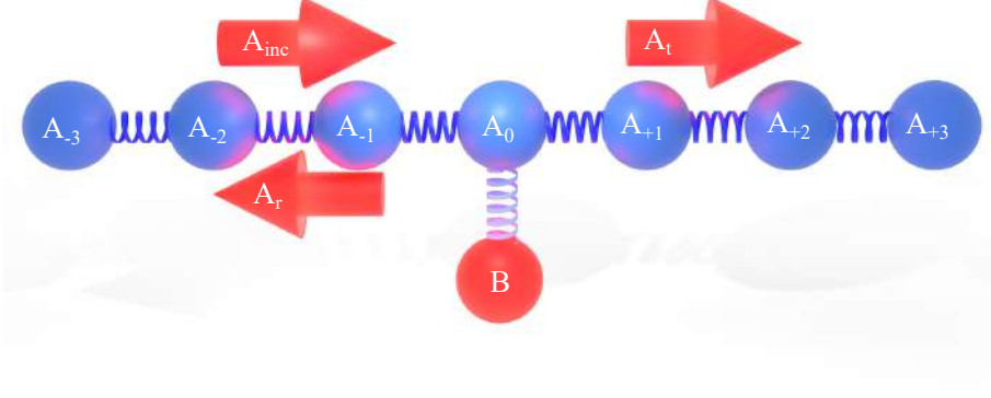
Figure 5.8: The model's concept of an oscillator chain, marking A_{\text{inc}} as incident wave and its reflected A_r and transmitted A_t waves. Additional central and side-coupled component ( B to A_0 ) is added as a perturbation, and such oscillator part represents the Fabry–Perot and guided-mode resonance of the thin-film structure.
