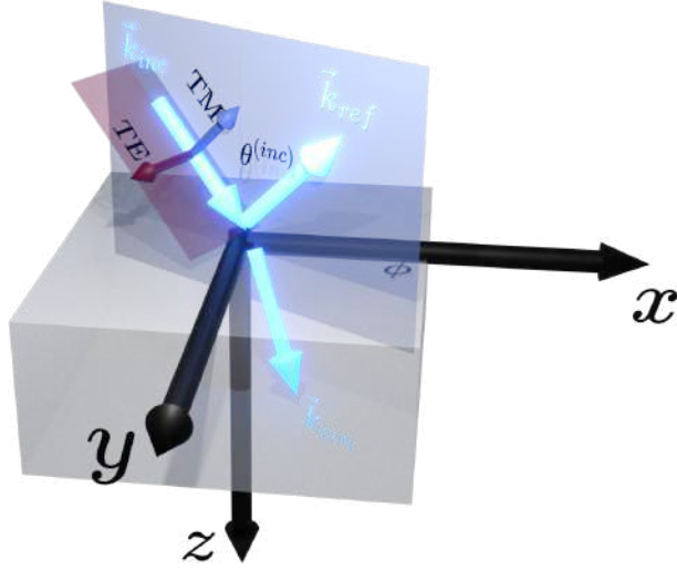
Figure 1.7: Polarization components in spherical coordinate system.
