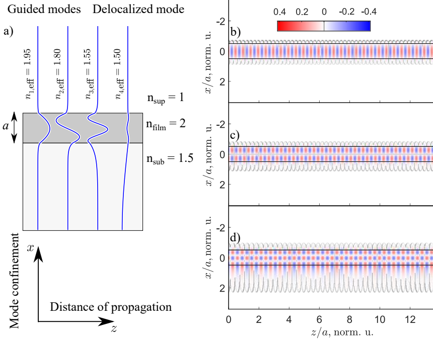
Figure 1.1: Representation of guided slab waveguide modes in 1D confinement. The modes are presented in (a) and their guided parts in (b-d) for TE polarization (H mode). The wavelength is \lambda_0 = 0.97\mu\text{m} and slab width a = 1\mu\text{m} .
