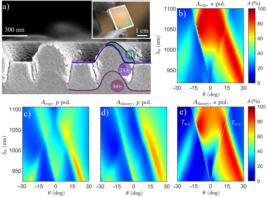
Figure 4.7: Experimental fabrication of doubly periodic GMR filter with an asymmetrical absorber (SEM picture) (a), indirect measurement of absorption for s polarized input (b) and p polarized input (c). Simulated spectra are presented in (d,e) [115].
