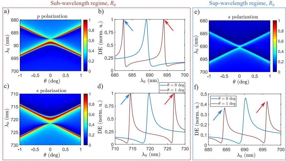
Figure 5.7: Zeroth order reflection spectra for the passive thin film GMR filter. Reflection is provided for p polarized input in a) and its resonances at \theta = 0 deg and \theta = 1 deg angle of incidence at b). Reflection is provided for s polarized input in c) and its resonances at \theta = 0 deg and \theta = 1 deg angle of incidence at d). Sup-wavelength regime of R_0 is provided for s polarized input in e) and its slices at \theta = 0 deg and \theta = 1 deg angle of incidence at f).
