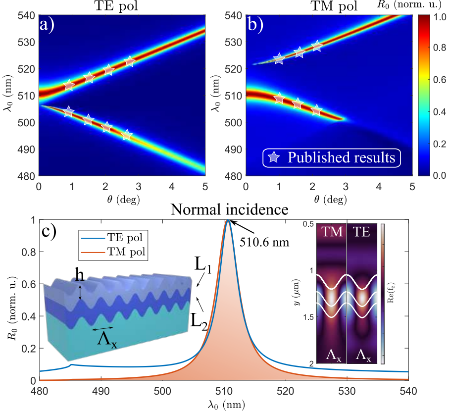
Figure 6.3: RCWA derived reflection spectra distributions of TE polarization (a), TM polarization (b) and their intersection at normal incidence (c) for double layered harmonic gratings first reported in [148].
