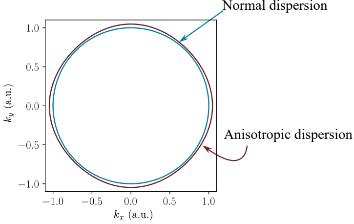
Figure 1.13: Dispersion comparison between the Normal dispersion and the Anisotropic one, given \Delta x = 1 and \Delta y = 1 a.u. for \varepsilon_r = \mu_r = 1 .
