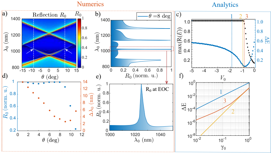
Figure 3.3: Reflection angular spectrum (a), and its cross-section at an oblique angle of incidence (b). The arrows indicate the points corresponding to the resonance at the EOC. The peak reflectance and its spectral width dependence vs potential well's depth V_0 analytical model. The peak reflectance and its spectral FWHM dependence on angle of incidence from RCWA model (d) and the zoomed in resonant reflection at e). The width dependence of the resonance from analytical study is present at f).
