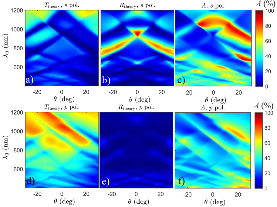
Figure 4.4: Doubly modulated GMR structure with the asymmetrical absorber. The transmission and reflection spectra for s polarization (a,b), absorption profile for s polarization (c), transmission and reflection spectra for p polarization (d,e) respectively and the absorbance for p polarization (f).
