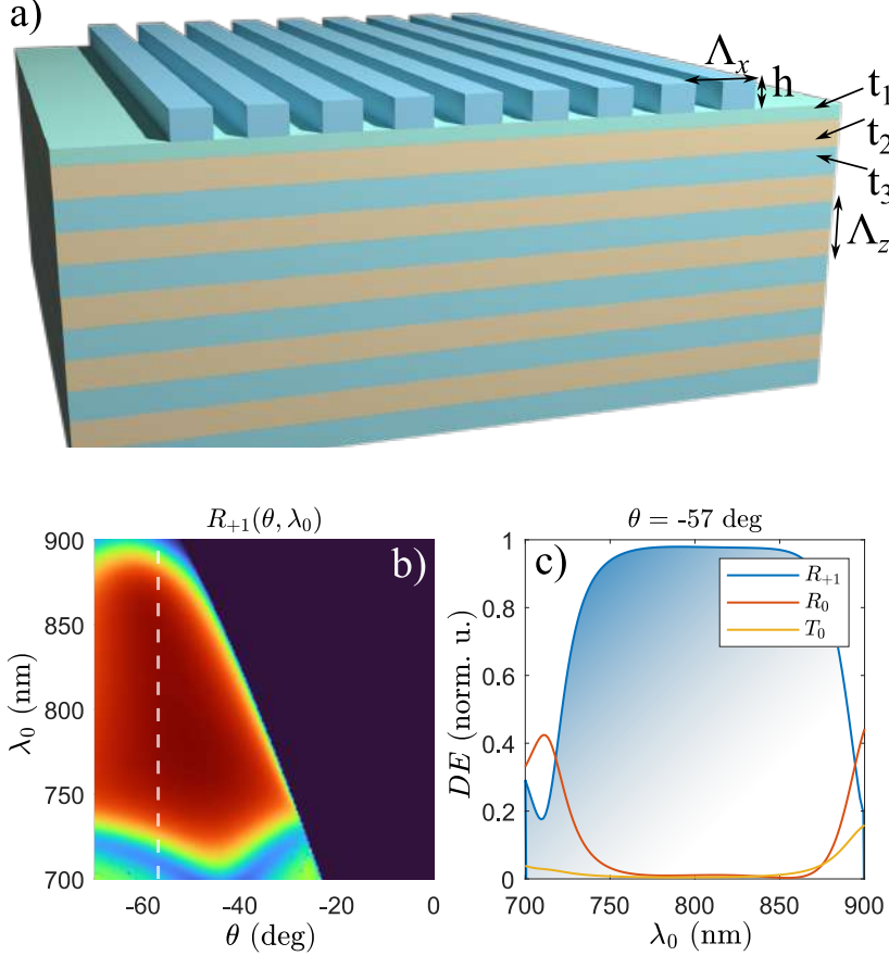
Figure 6.5: Flat top dispersive reflector spectrum [55]. a) denotes a device of interest with its geometrical parameters, b) its first-order reflection coefficient and c) diffraction order distribution.
